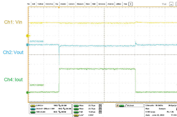
Figure 22. Load transient
