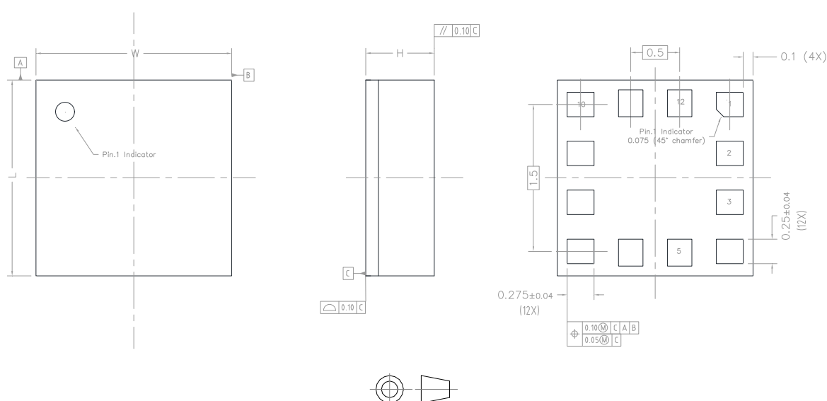
Figure 19. LGA-12L 2.0 x 2.0 x 0.74 mm package outline and mechanical data
