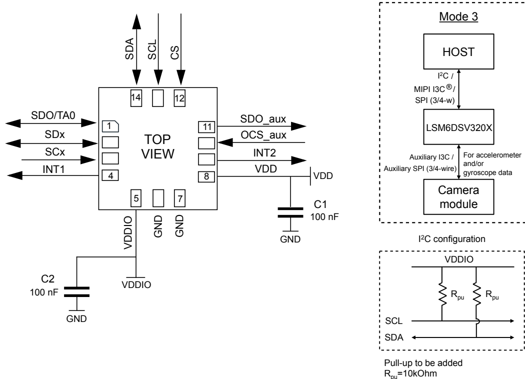
Figure 29. LSM6DSV320X electrical connections in mode 3 (auxiliary 3/4-wire SPI or auxiliary MIPI I3C)
