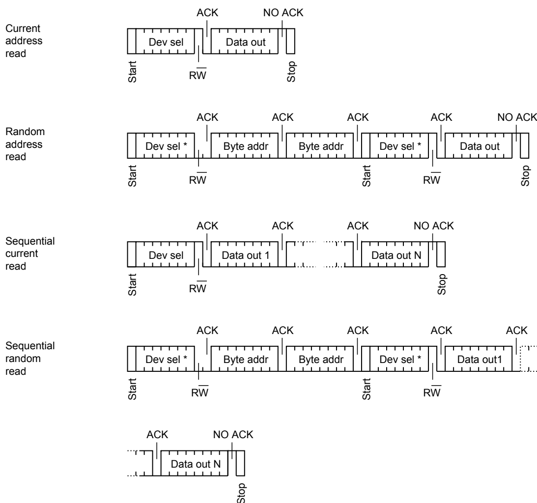
Figure 18. Read mode sequences
