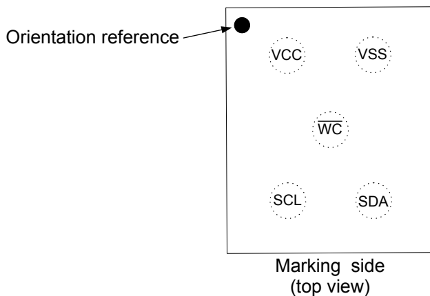
Figure 4. 5-ball package connection- WLCSP (CP)
