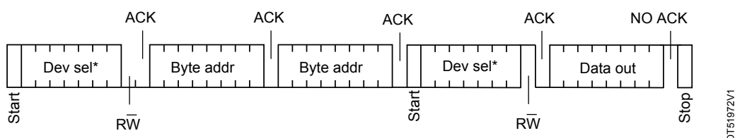
Figure 19. Random read DTI register
