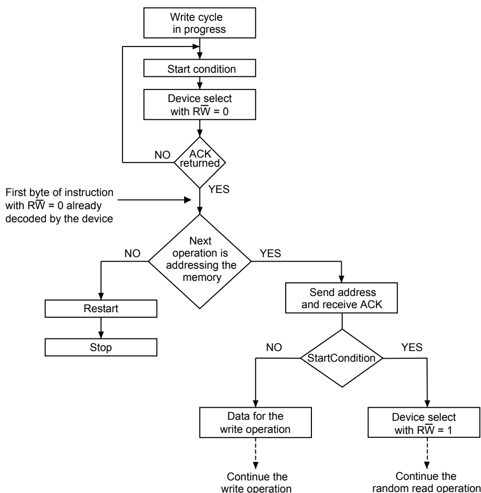
Figure 17. Write cycle polling flowchart using ACK
