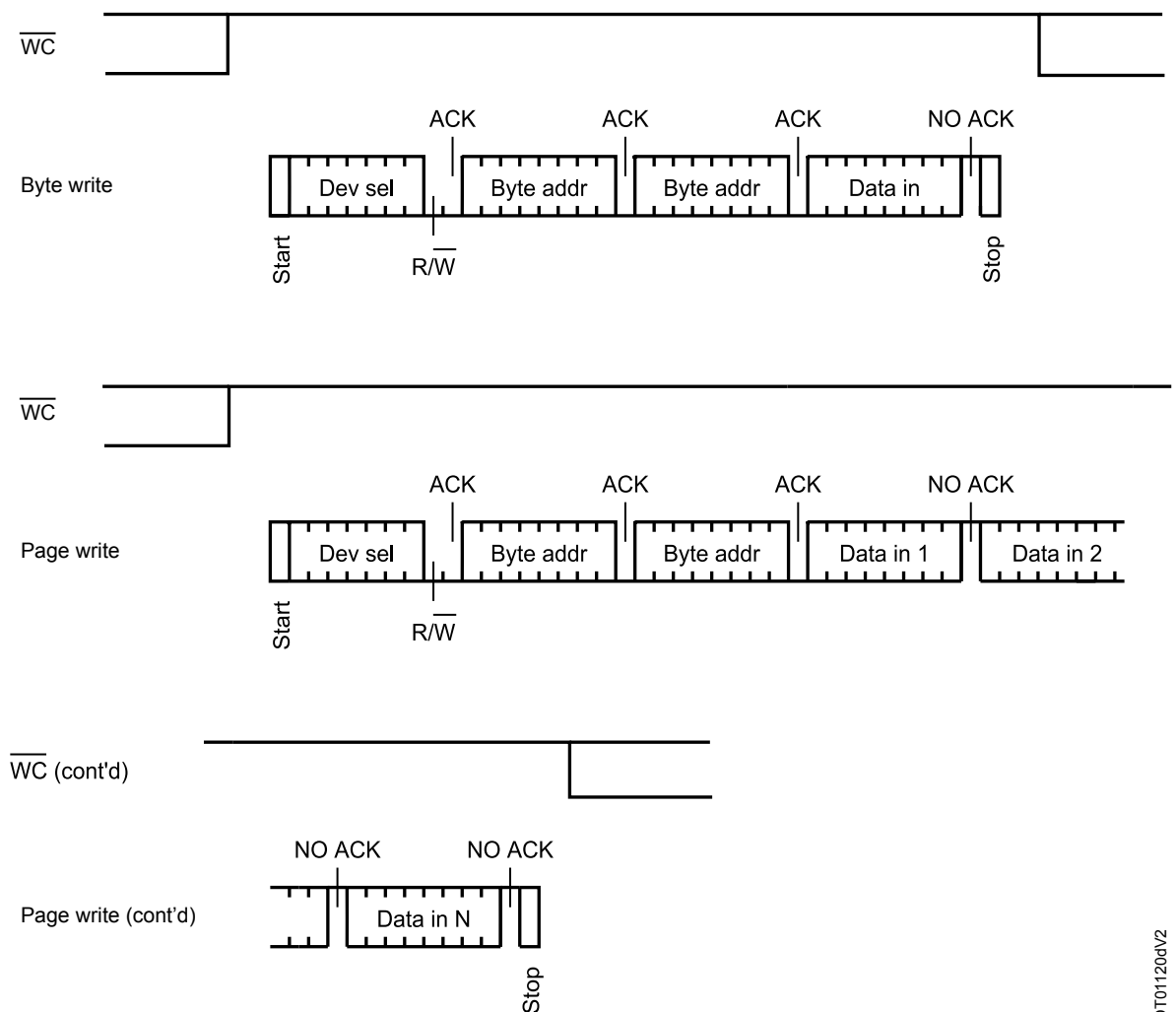
Figure 8. Write mode sequences with write protection (data write inhibited)
