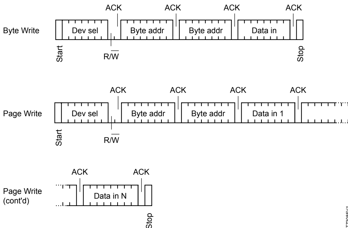
Figure 13. Write identification page (page unlocked)
