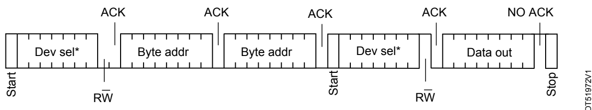
Figure 20. Random read CDA register
