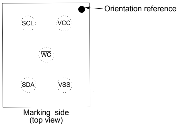
Figure 3. 5-ball package connection - WLCSP (CS)
