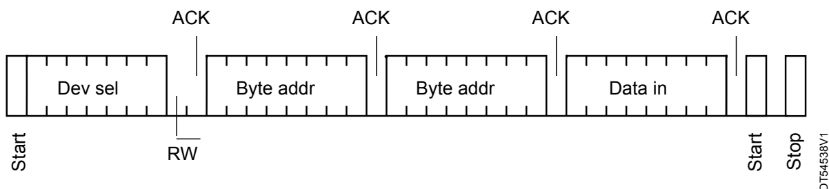
Figure 24. Read lock status (identification page locked)
