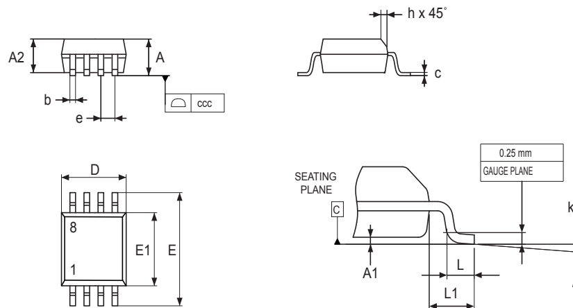
Figure 29. SO8N - Outline
