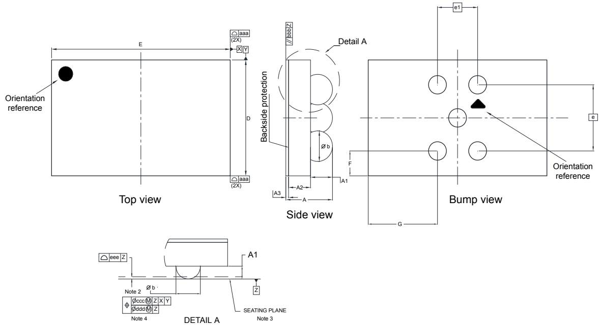
Figure 36. WLCSP5 (CP) with BSC - Outline
