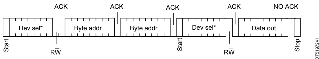
Figure 21. Random read SWP register
