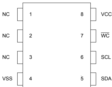
Figure 2. 8-pin package connections, top view
