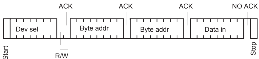
Figure 10. Write CDA register (data write inhibited by software or hardware)
