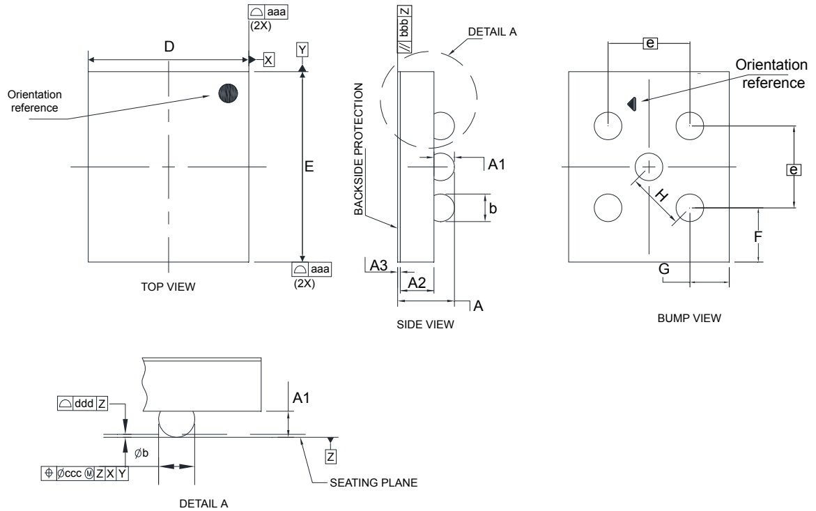
Figure 35. WLCSP5 (CS) with BSC - Outline
