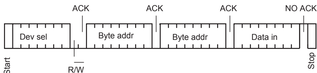
Figure 12. Write SWP register (data write inhibited by software or hardware)
