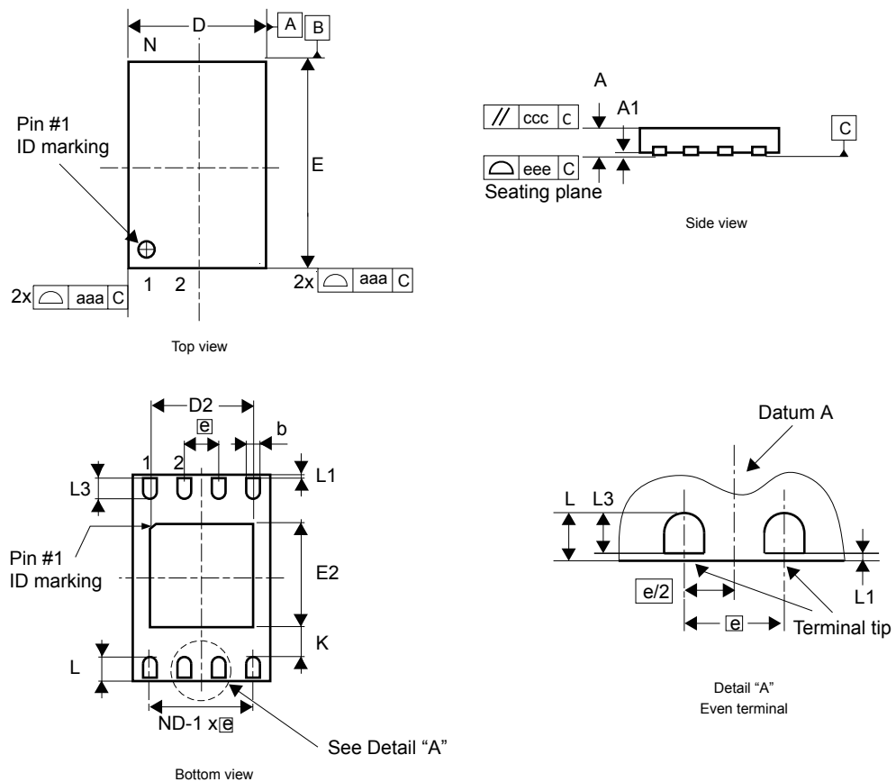
Figure 33. UFDFPN8 - Outline
