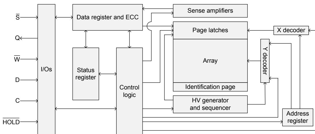
Figure 3. Block diagram
