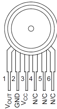
Pinout
