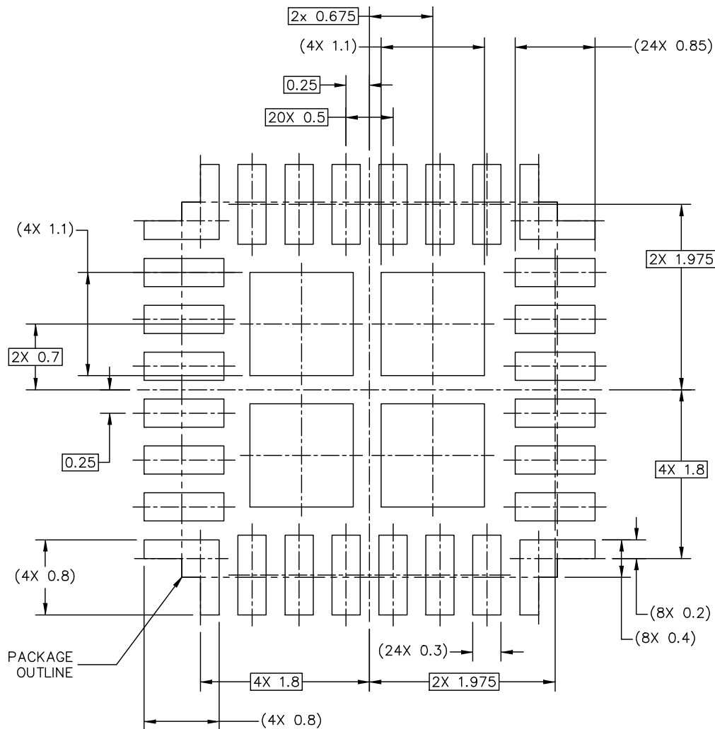
Figure 12. Reflow soldering footprint part3 for HQFN24 (SOT1931-1(D))
