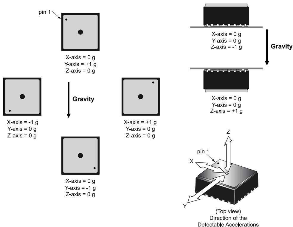
Figure 3. NTM88Hxx5S orientation at rest
