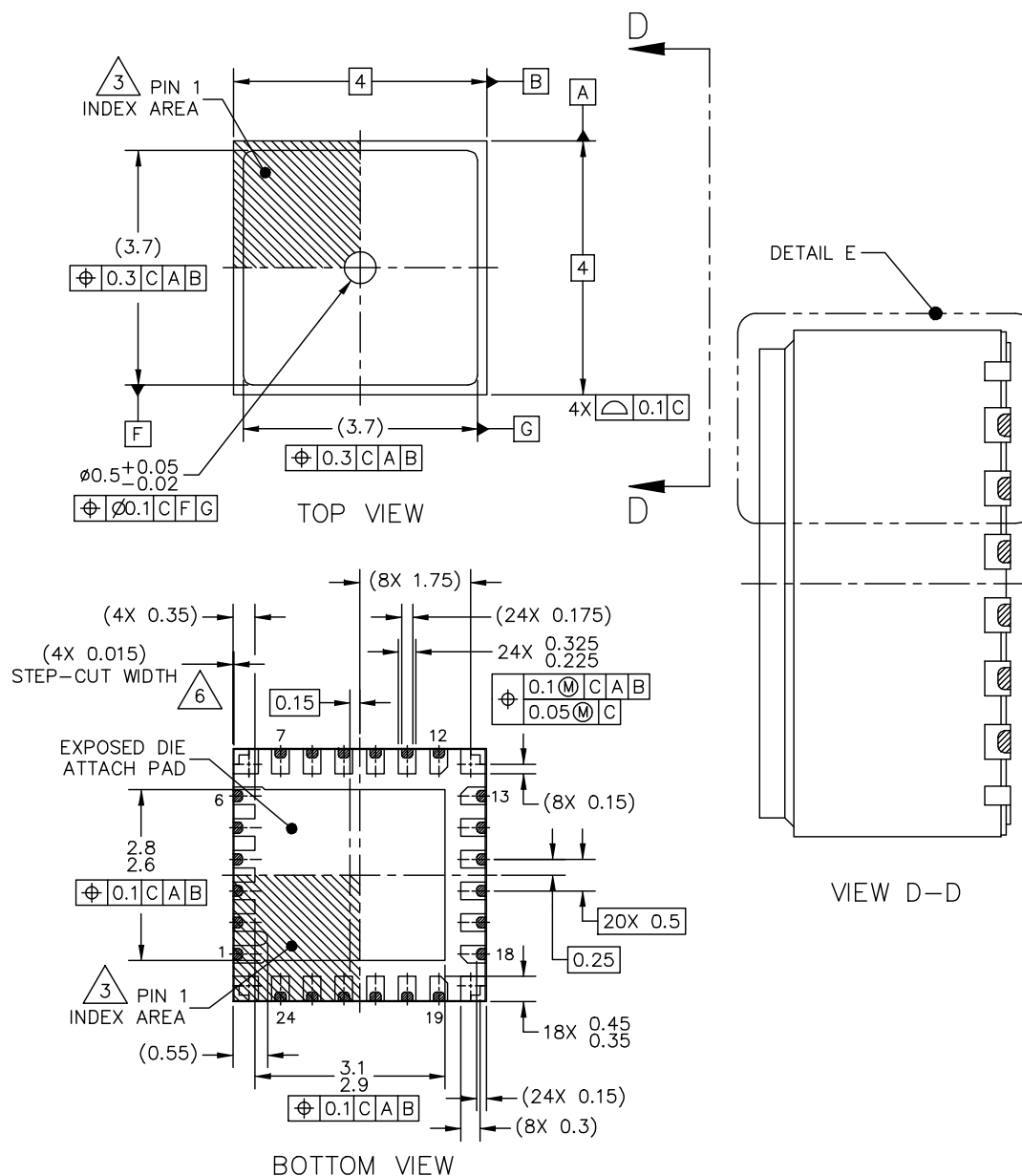
Figure 8. Package outline HQFN24 (SOT1931-1(D))
