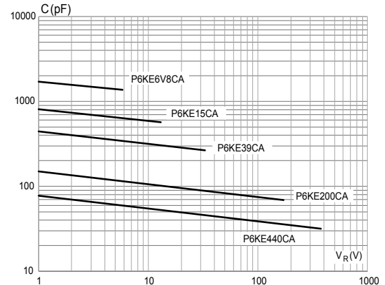
Figure 8. Junction capacitance versus applied voltage (bidirectional type)
