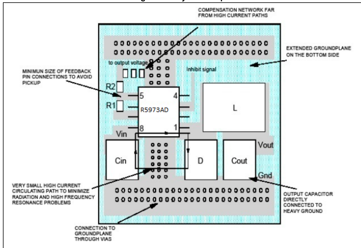
Figure 13. Layout example
