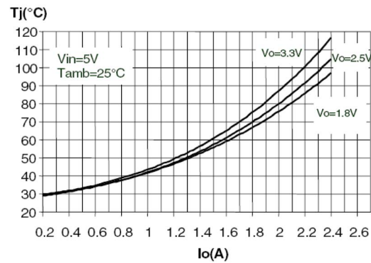
Figure 28. Junction temperature vs. output current - V_{IN} = 5\text{ V}
