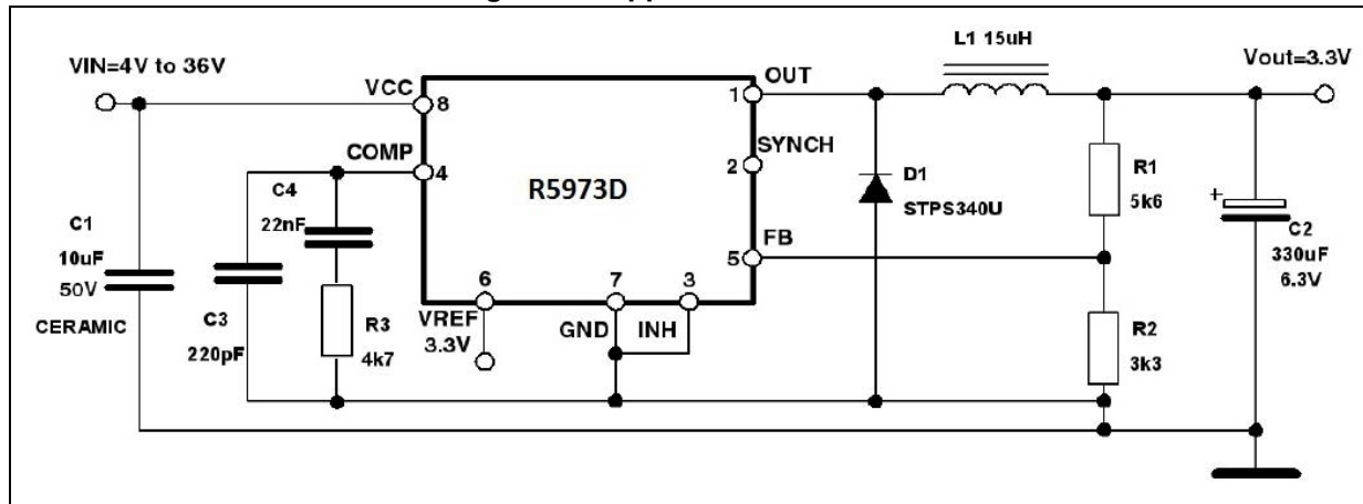
Figure 12. Application schematic
