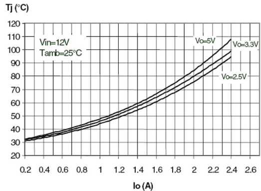
Figure 29. Junction temperature vs. output current - V_{IN} = 12\text{ V}
