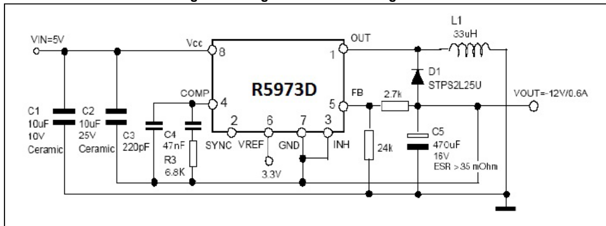
Figure 19. Negative buck-boost regulator
