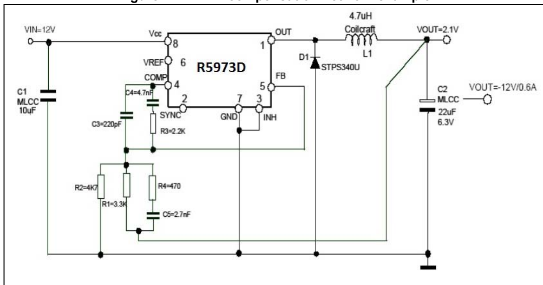
Figure 21. MLCC compensation network example
