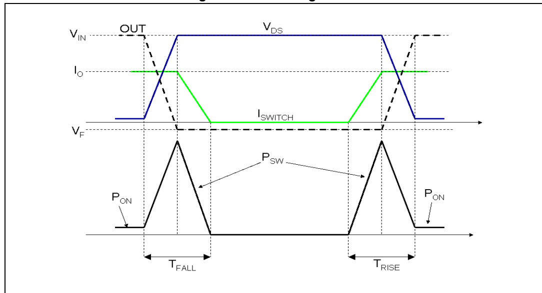
Figure 14. Switching losses
