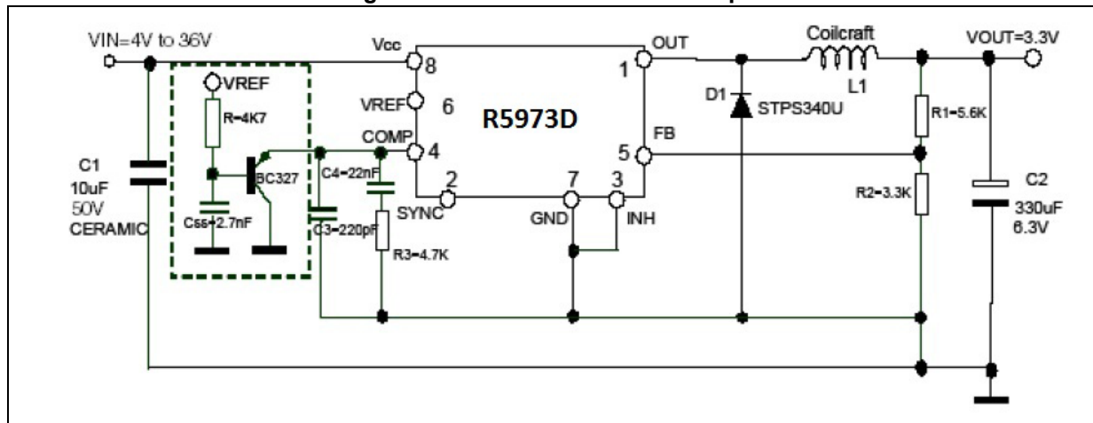
Figure 22. Soft-start network example
