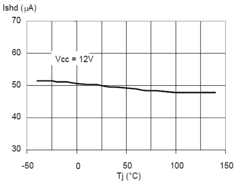
Figure 24. Shutdown current vs. junction temperature
