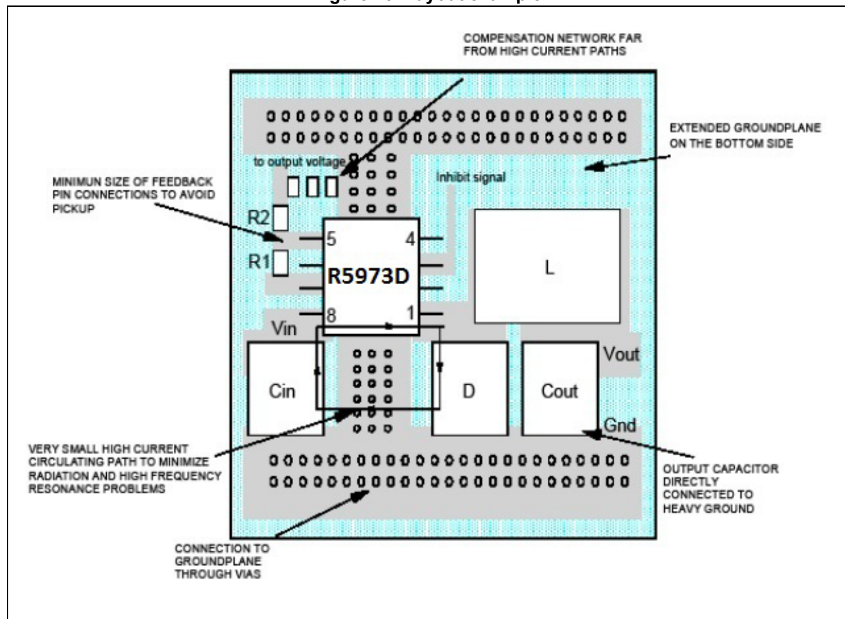
Figure 13. Layout example
