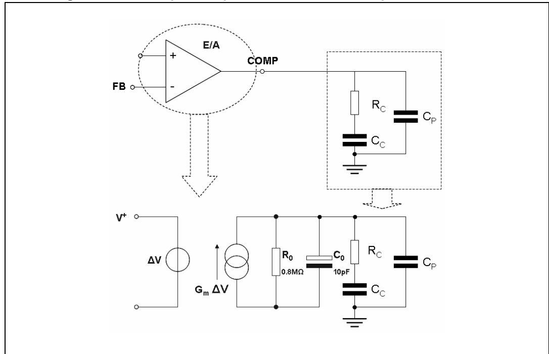
Figure 9. Error amplifier equivalent circuit and compensation network
