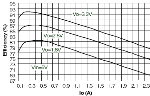
Figure 30. Efficiency vs. output current - V_{IN} = 5\text{ V}
