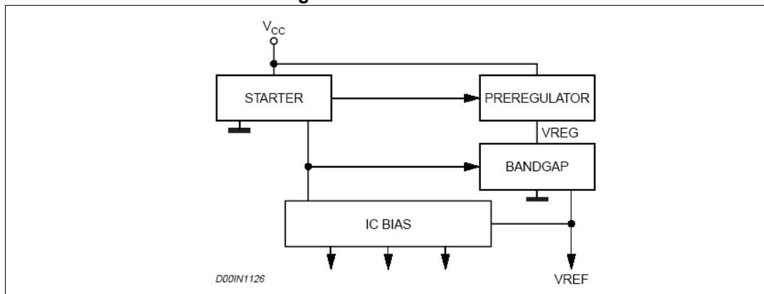
Figure 3. Internal circuit
