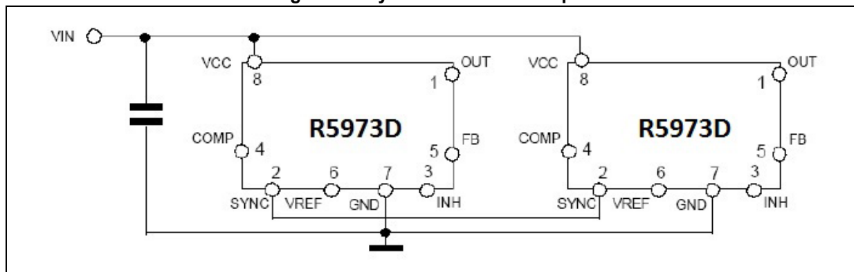
Figure 20. Synchronization example
