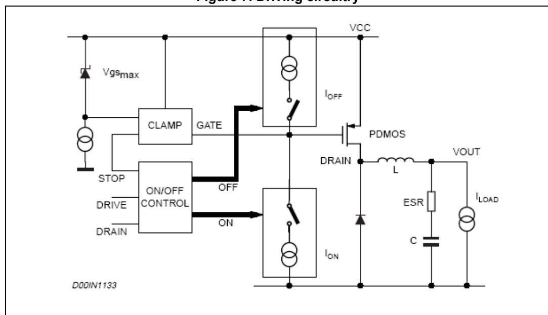
Figure 7. Driving circuitry
