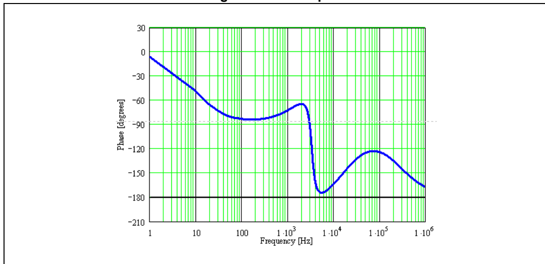
Figure 11. Phase plot
