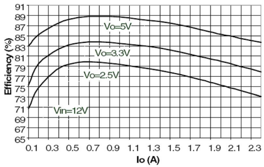
Figure 31. Efficiency vs. output current - V_{IN} = 12\text{ V}
