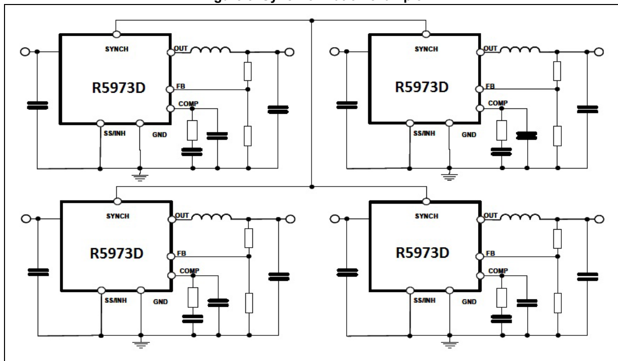
Figure 5. Synchronization example
