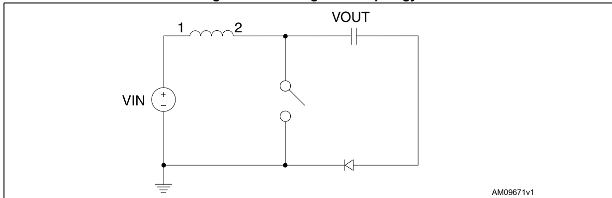
Figure 24. Floating boost topology
