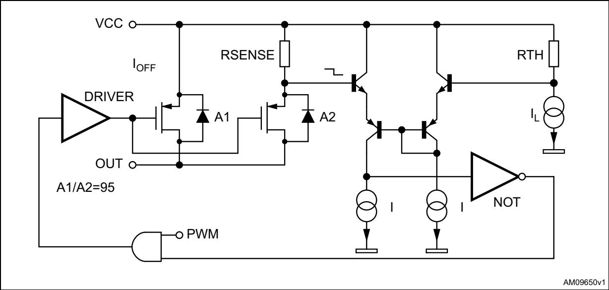
Figure 6. Current limitation circuitry
