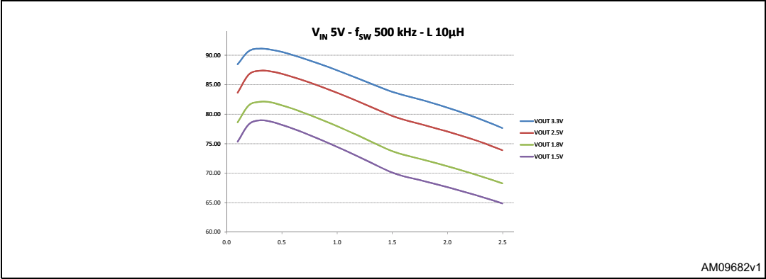
Figure 35. Efficiency vs. output current ( V_{IN} = 5\text{ V} )
