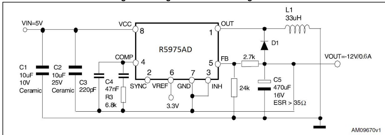
Figure 23. Negative buck-boost regulator
