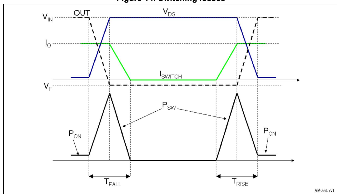
Figure 14. Switching losses
