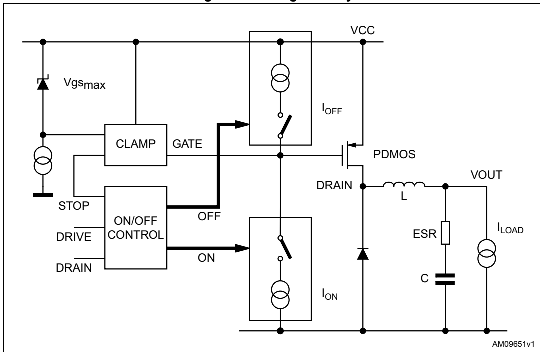
Figure 7. Driving circuitry
