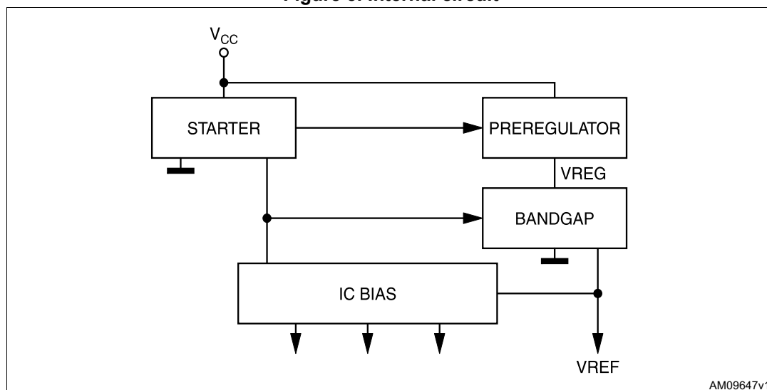
Figure 3. Internal circuit
