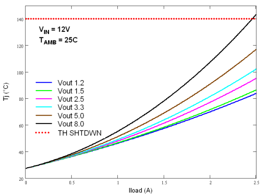
Figure 33. Junction temperature vs. output current ( V_{IN} = 12V )
