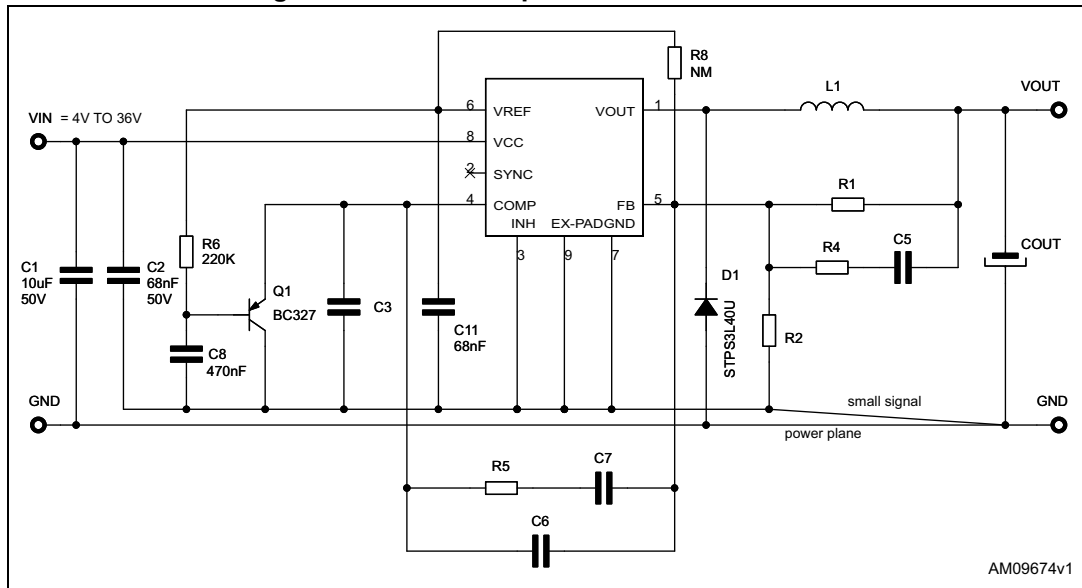
Figure 27. MLCC compensation network circuit
