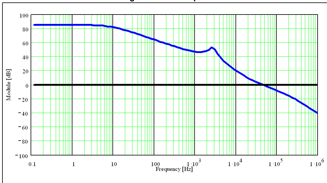
Figure 10. Module plot
