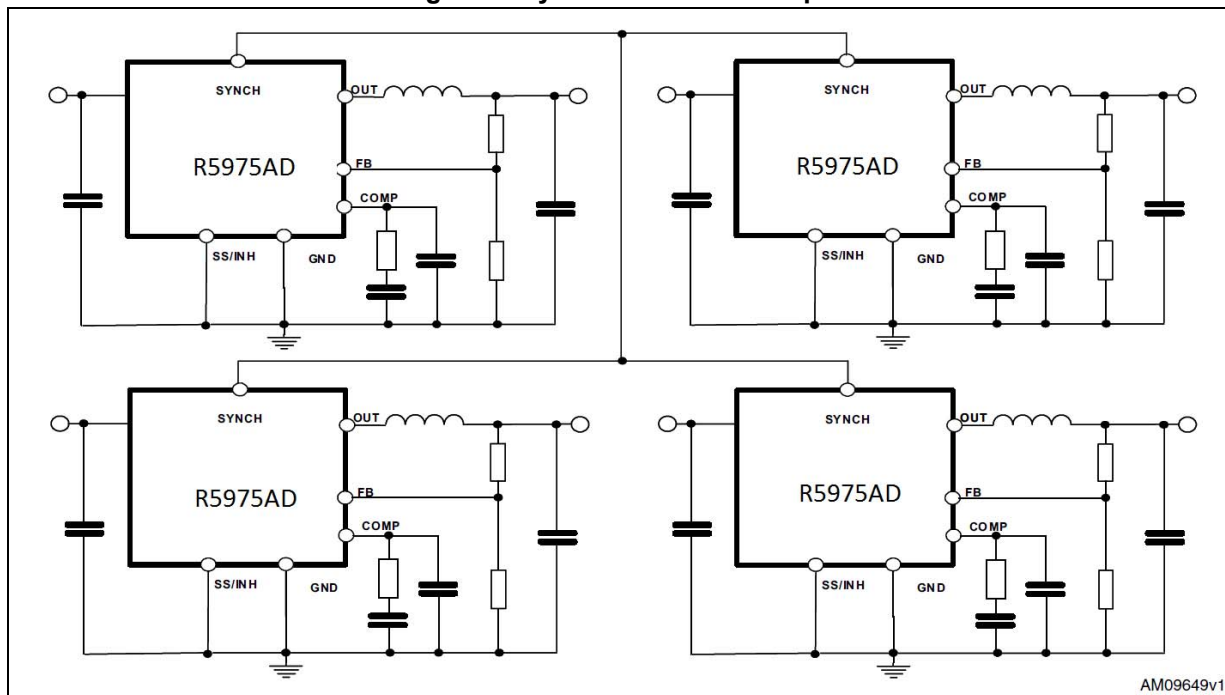
Figure 5. Synchronization example
