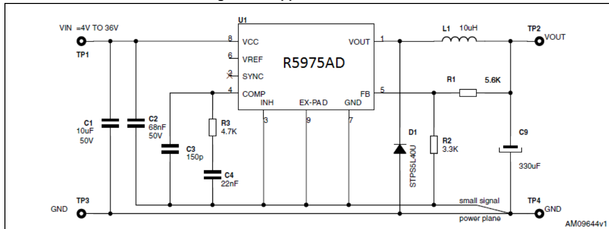
Figure 12. Application schematic
