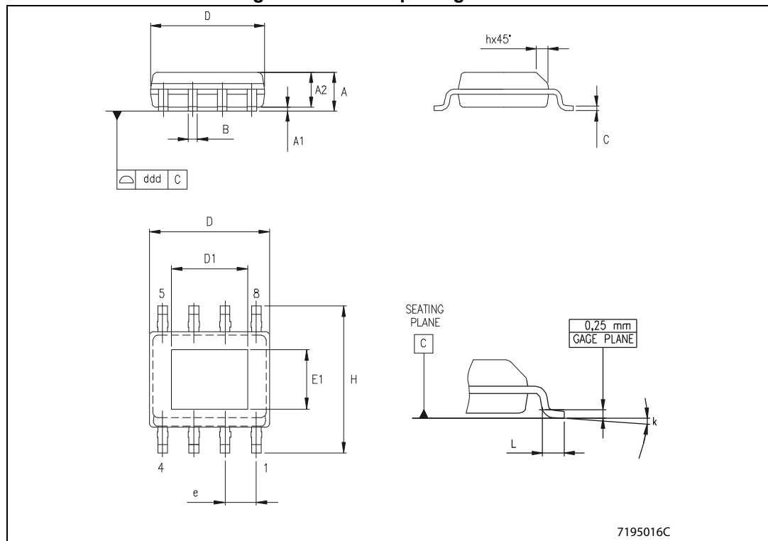
Figure 36. HSOP8 package outline
