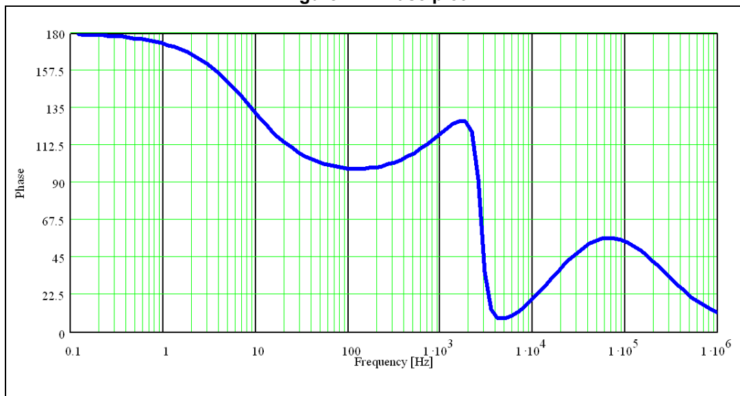
Figure 11. Phase plot
