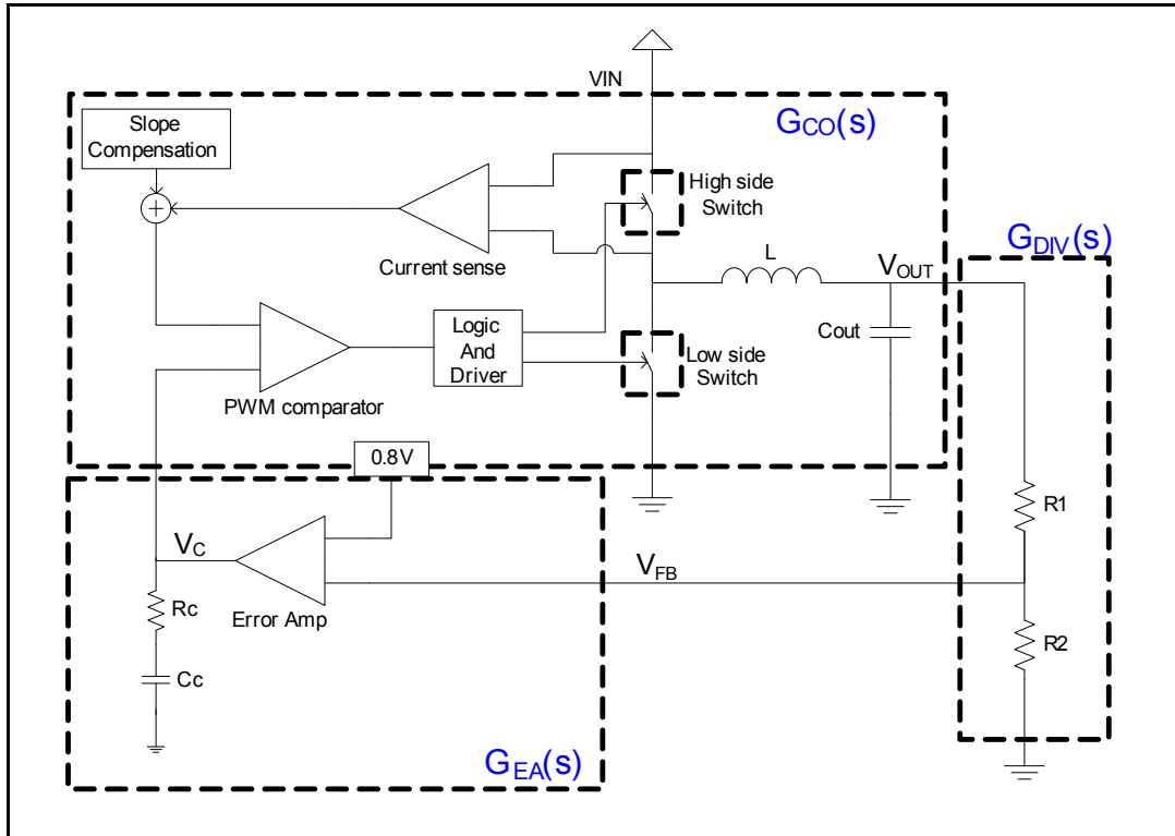
Figure 3. Block diagram of the loop for the small signal analysis
