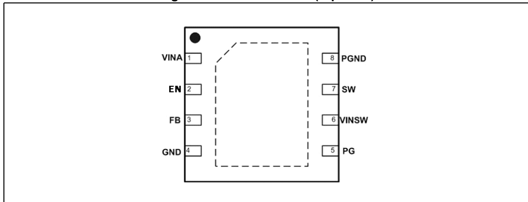
Figure 1. Pin connection (top view)
