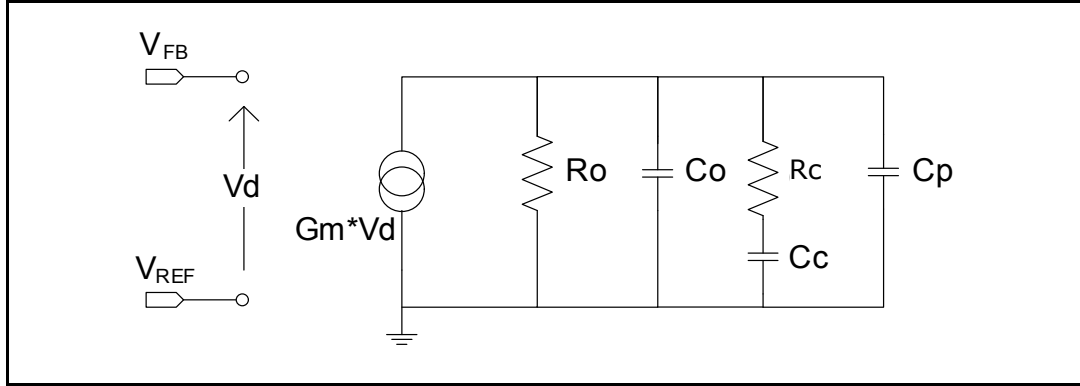
Figure 4. Small signal model for the error amplifier
