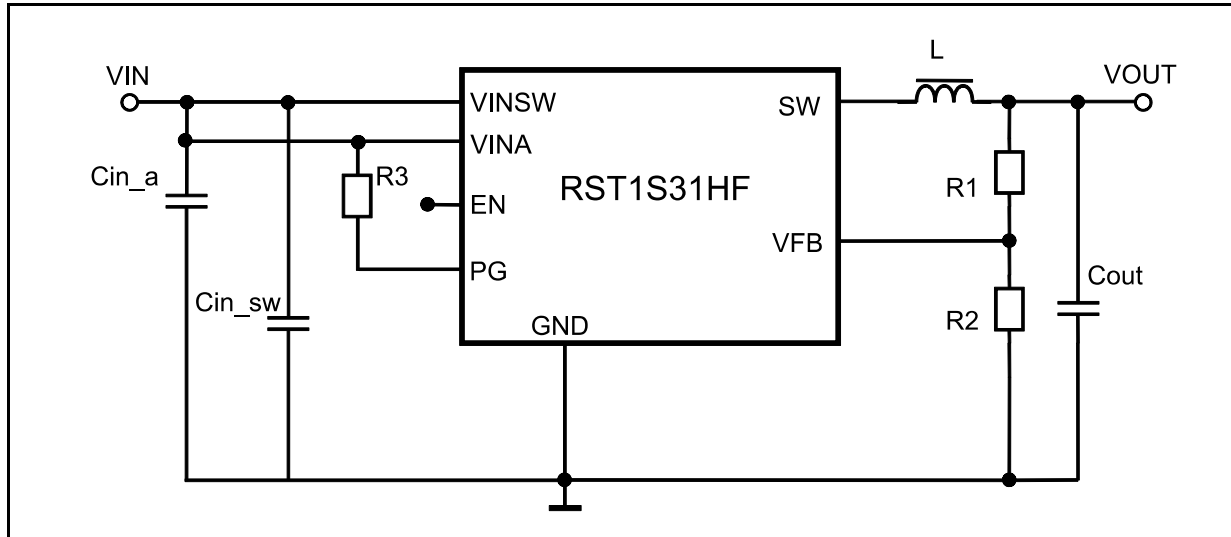
Figure 7. Application circuit
