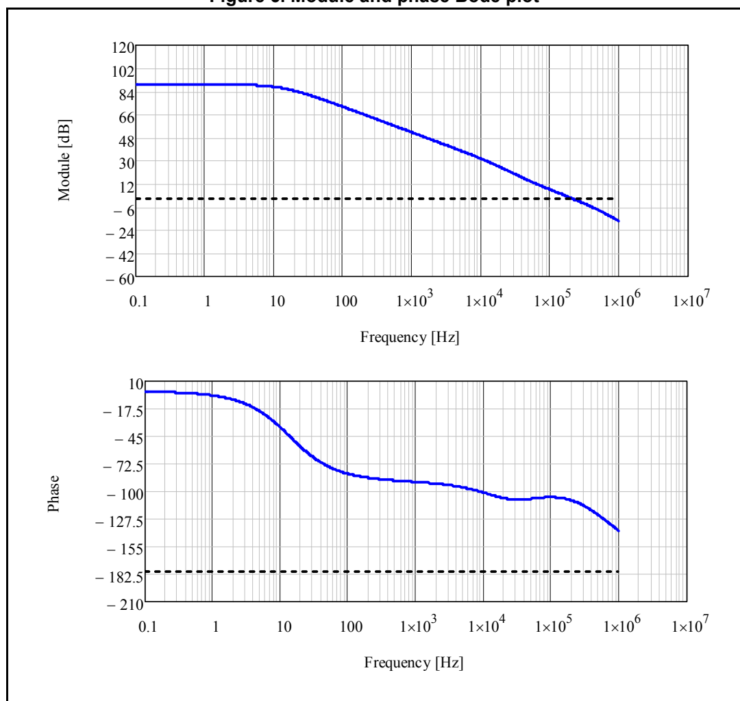
Figure 5. Module and phase Bode plot
