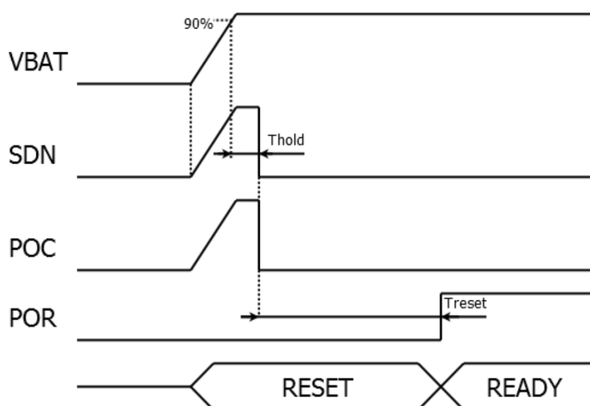
Figure 7. Start-up phase
