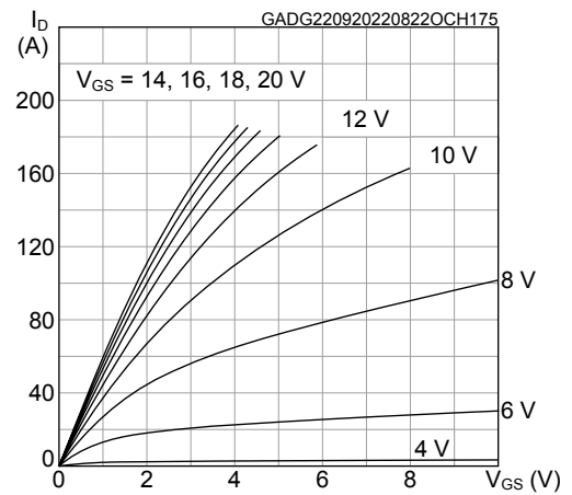
Figure 4. Typical output characteristics ( T_J = 175\text{ °C} )
