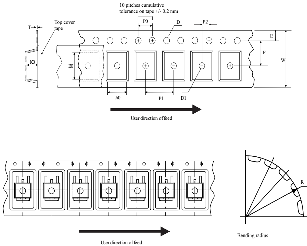
Figure 21. Tape outline
