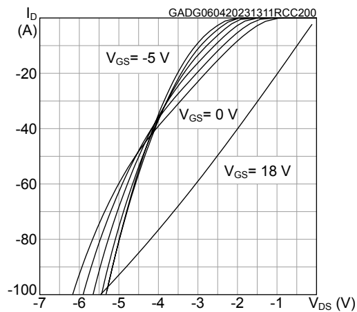
Figure 17. Typical reverse conduction characteristics ( T_J = 200 \text{ }^\circ\text{C} )
