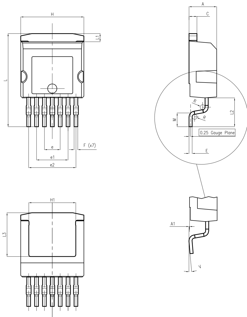
Figure 16. H 2 PAK-7 package outline
