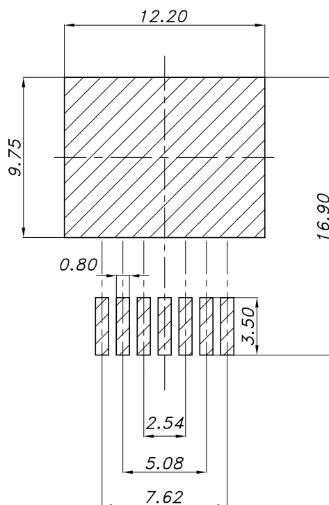
Figure 17. H 2 PAK-7 recommended footprint
