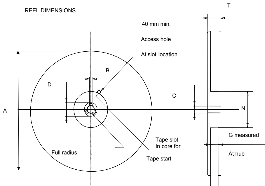
Figure 19. Reel outline
