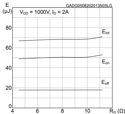
Figure 11. Typical switching energy vs R_G
