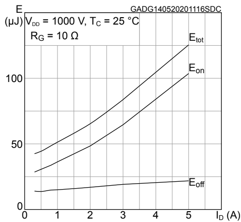
Figure 9. Typical switching energy vs I_D
