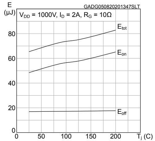
Figure 10. Typical switching energy vs temperature
