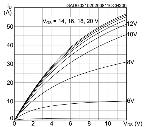
Figure 4. Typical output characteristics ( T_J = 200\text{ °C} )
