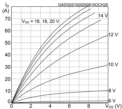
Figure 3. Typical output characteristics ( T_J = 25\text{ °C} )
