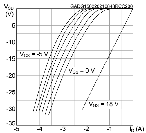
Figure 16. Typical reverse conduction characteristics ( T_J = 200^\circ\text{C} )
