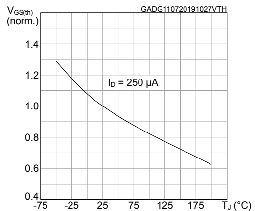
Figure 12. Normalized gate threshold vs temperature
