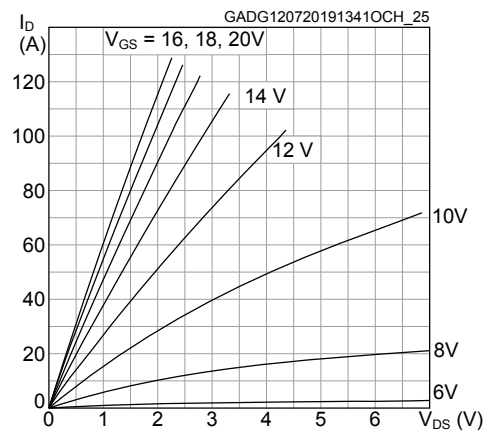
Figure 4. Typical output characteristics ( T_J = 25\text{ °C} )
