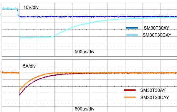
Figure 13. ISO7637-2 pulse 1a response ( V_S = -150\text{ V} ) with 12 V battery
