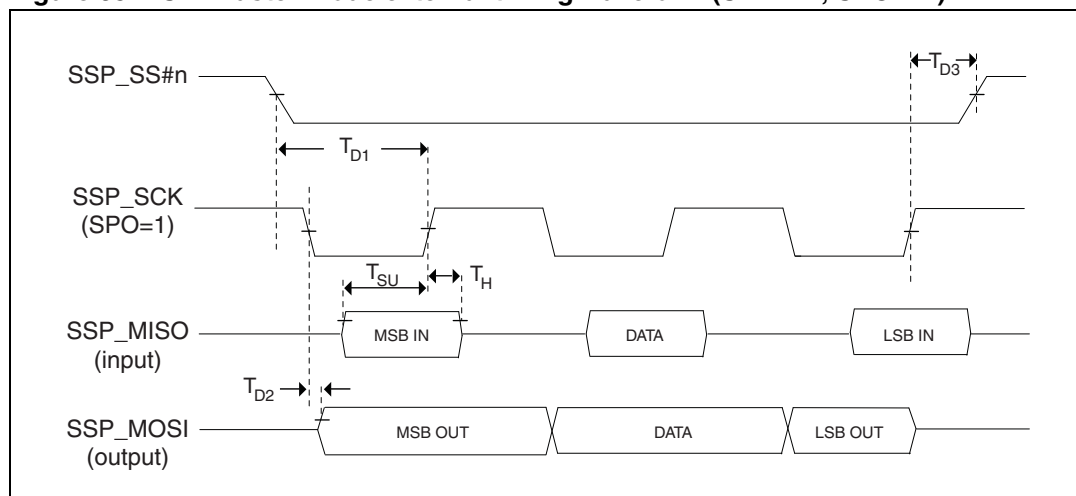
Figure 35. SPI master mode external timing waveform (SPH = 1, SPO = 1)
