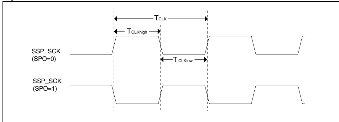
Figure 31. SSP_SCK waveform
