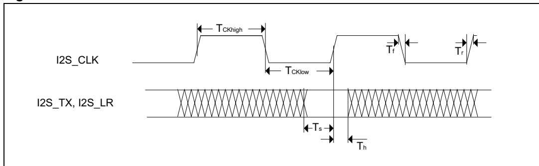
Figure 27. I2S waveform
