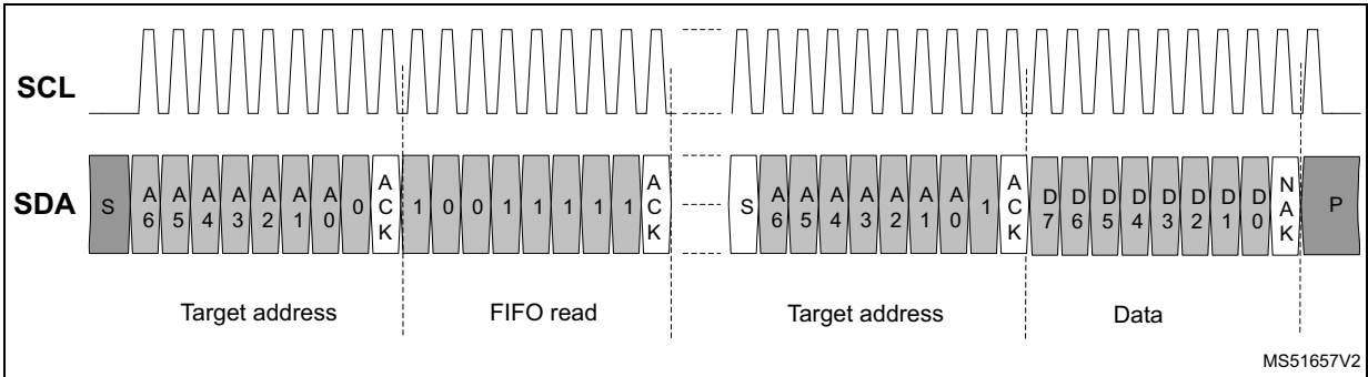
Figure 24. FIFO read
