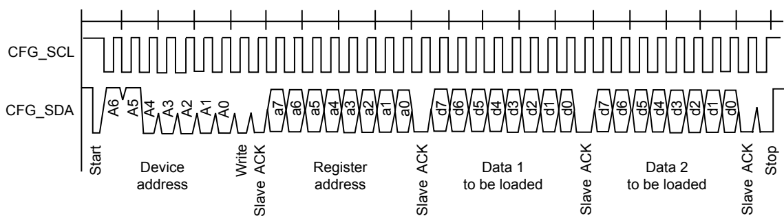
Figure 21. I 2 C write access
