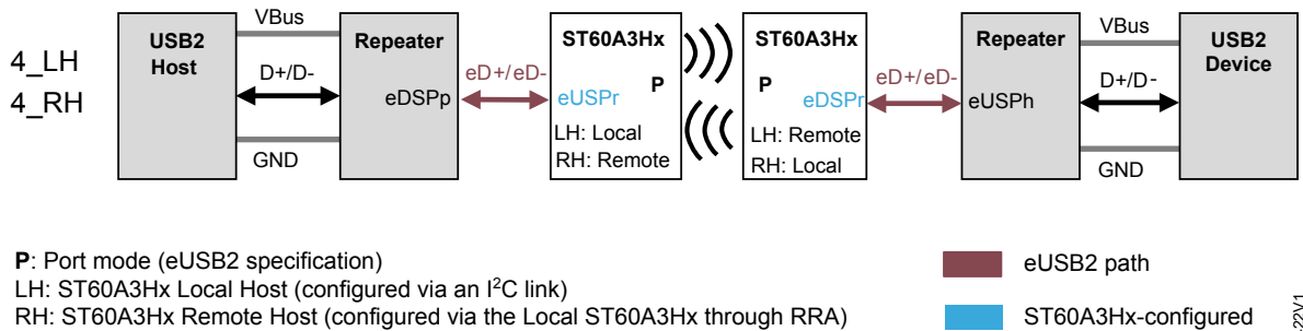
Figure 5. eUSB2 Hybrid Repeater configurations
