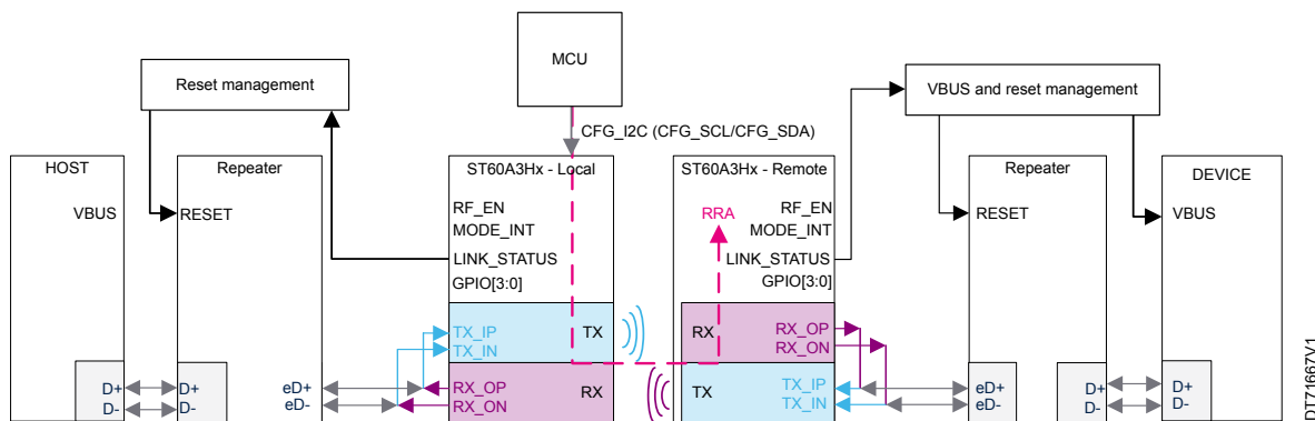
Figure 6. ST60A3H1 eUSB2 4_LH configuration
