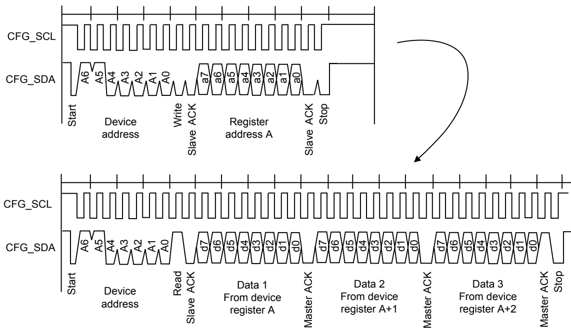
Figure 22. I 2 C read access
