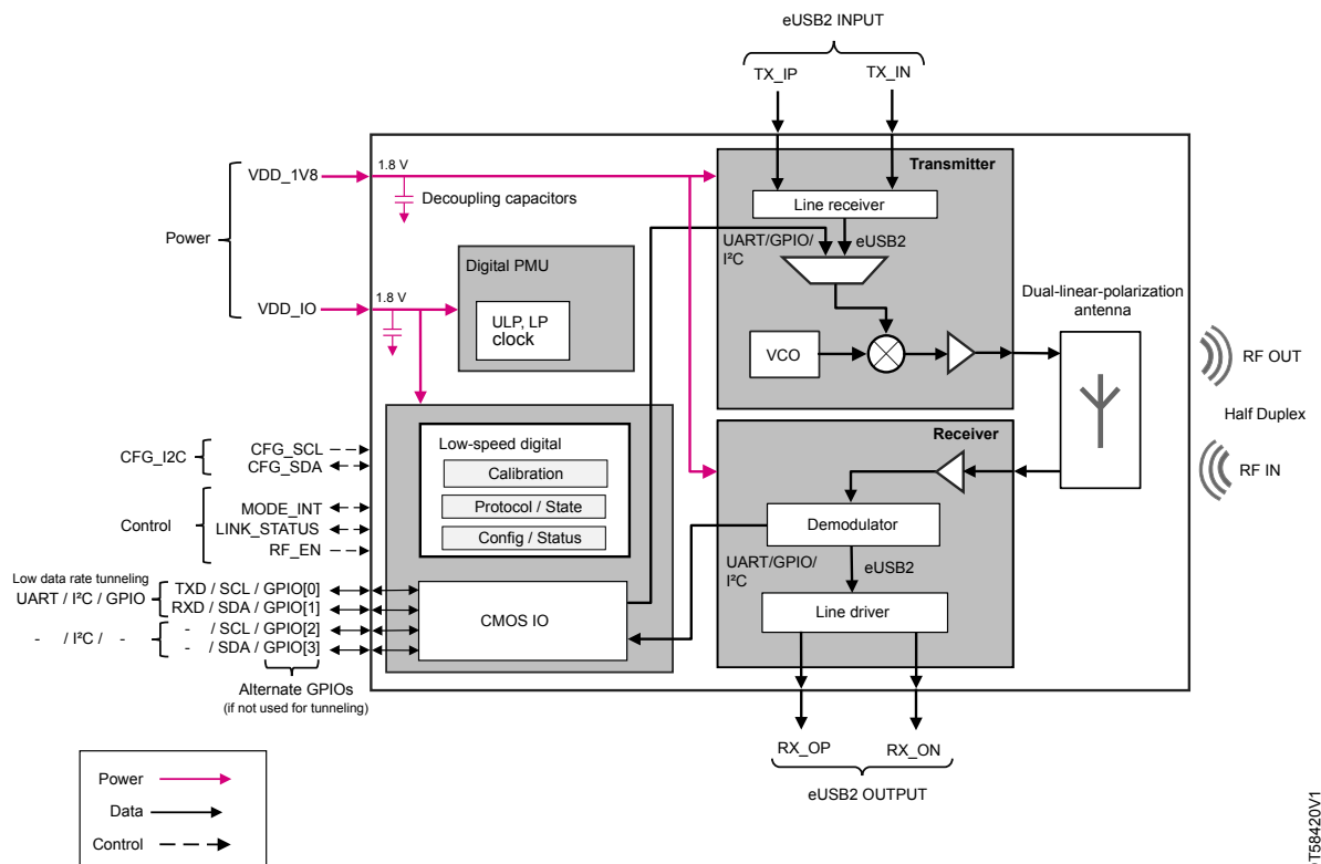
Figure 1. ST60A3H1 block diagram
