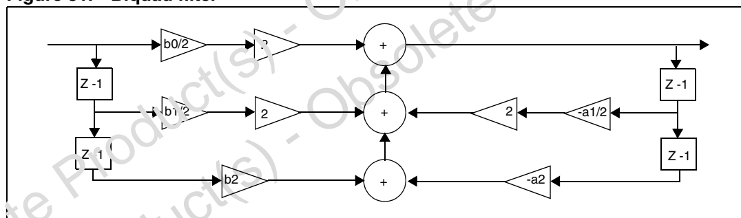
Figure 51. Biquad filter
