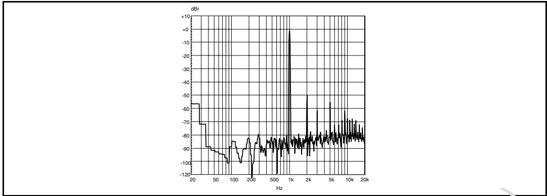
Figure 40. FFT 0 dB, 1 kHz, single ended, 3 Ω
