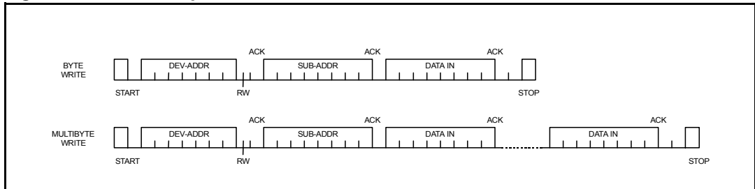
Figure 46. I 2 C write procedure
