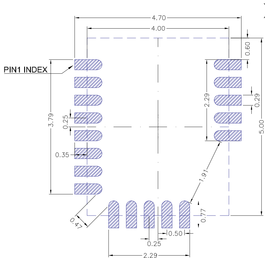
Figure 19. QFN 4 x 5 x 1 mm, 18 leads, 0.5 mm pitch, suggested footprint
