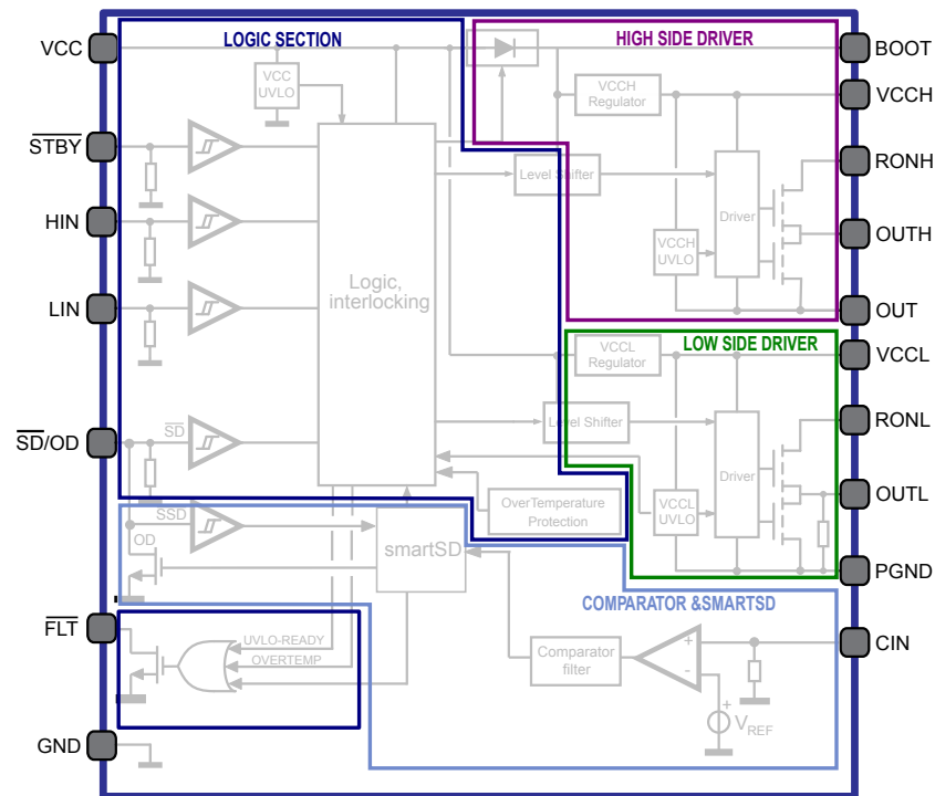
Figure 10. STDRIVEG211 simplified block diagram
