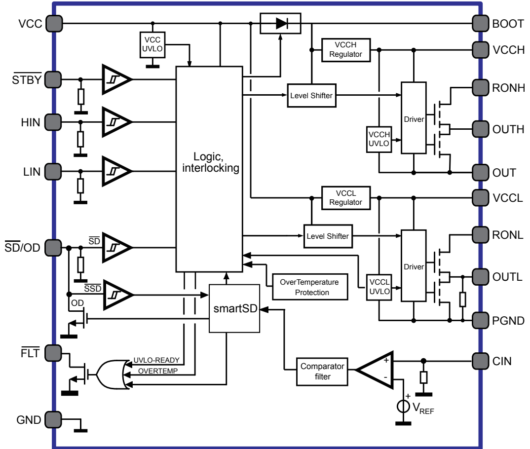
Figure 1. STDRIVEG211 block diagram
