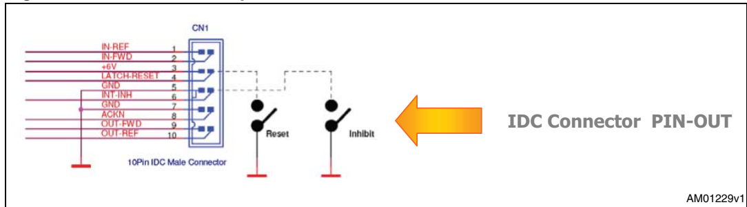
Figure 5. IDC connector piuout
