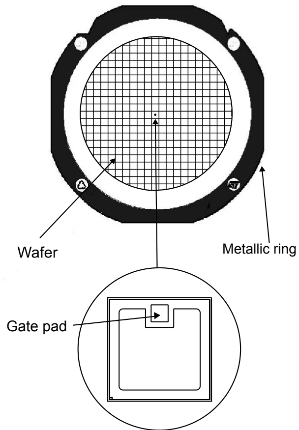
Figure 2. D7 drawing and die orientation
