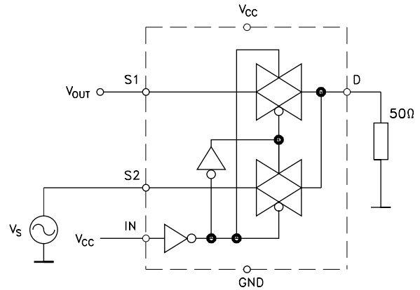
Figure 8. Channel-to-channel crosstalk
