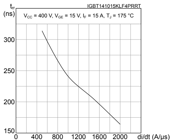
Figure 23. Typical reverse recovery time vs diode current slope
