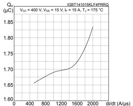
Figure 24. Typical reverse recovery charge vs diode current slope
