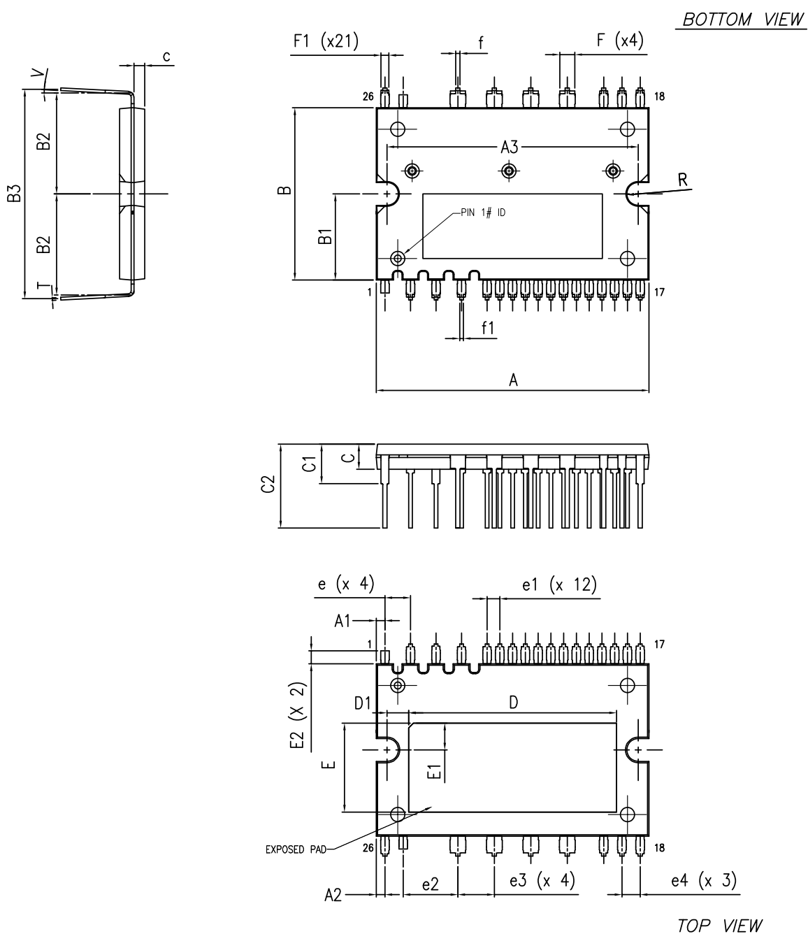
Figure 16. SDIP2B-26L type X2 package outline
