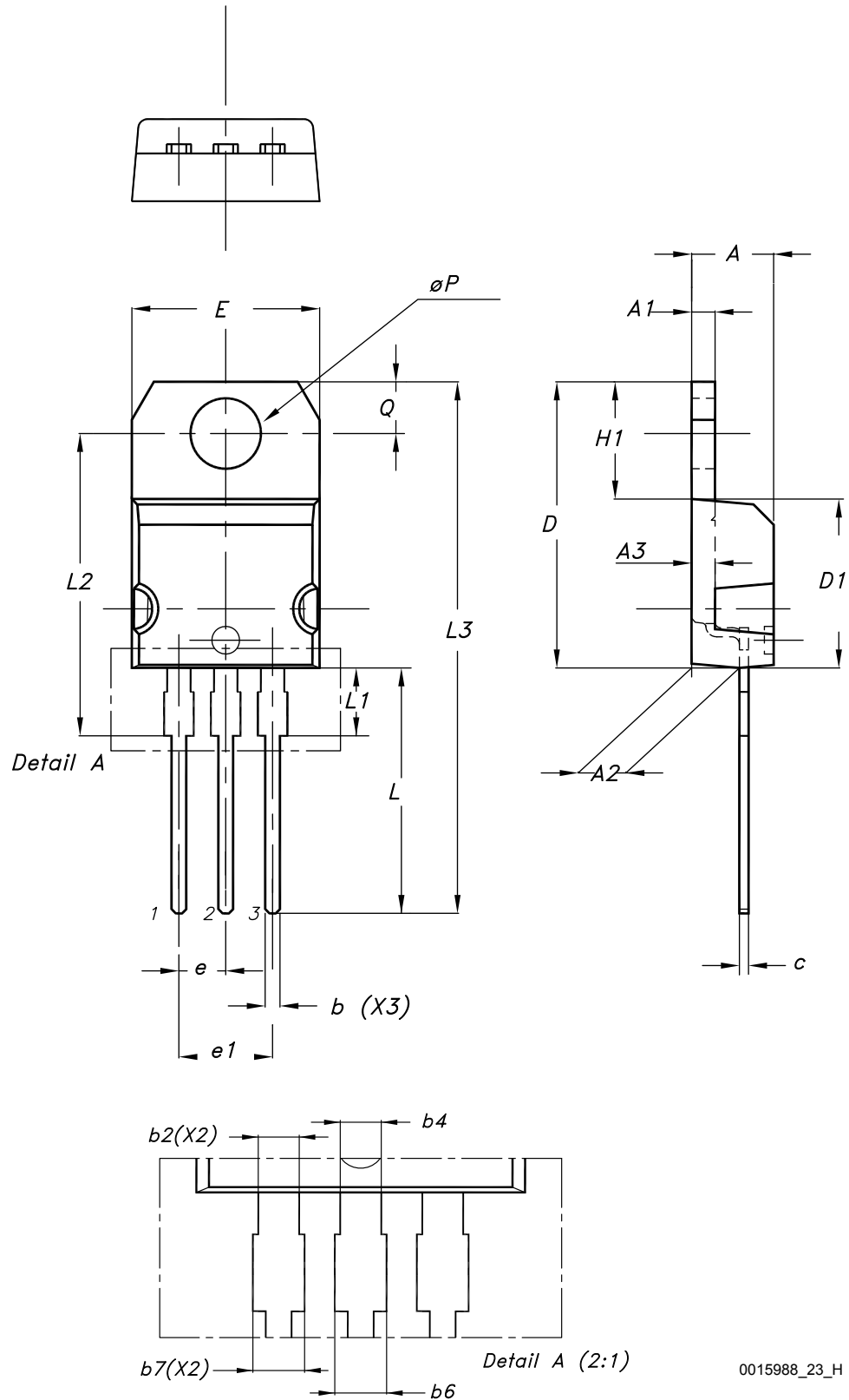
Figure 25. TO-220 type H package outline
