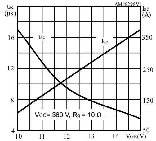
Figure 14. Short-circuit time and current vs V_{GE}
