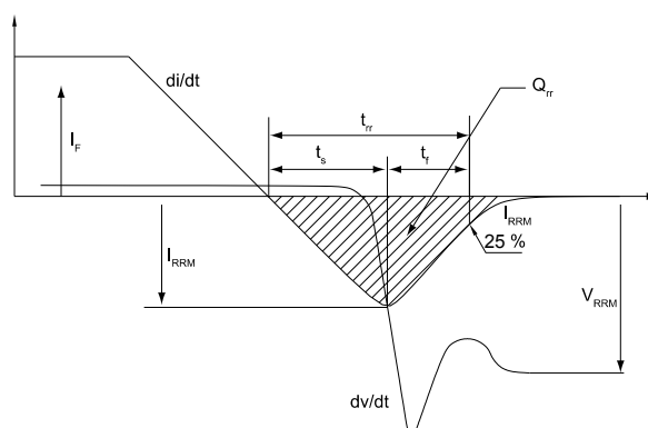
Figure 22. Diode reverse recovery waveform
