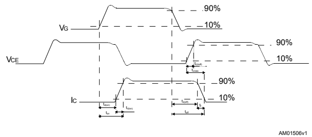
Figure 24. Switching waveform
