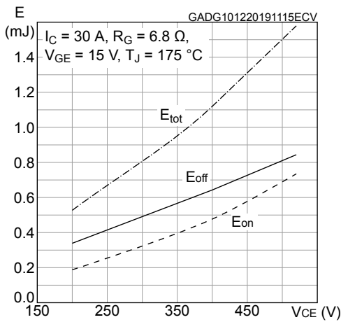
Figure 17. Switching energy vs collector emitter voltage
