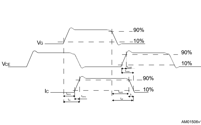
Figure 27. Switching waveform
