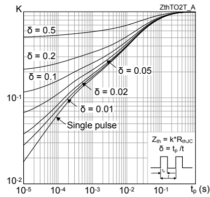
Figure 25. Thermal impedance for IGBT
