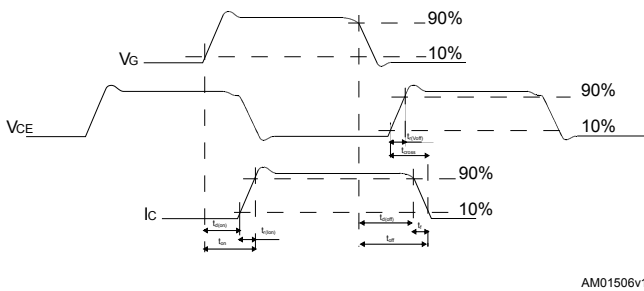
Figure 29. Switching waveform
