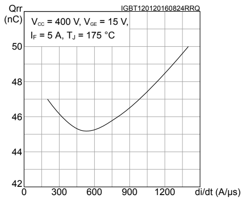
Figure 21. Reverse recovery charge vs diode current slope
