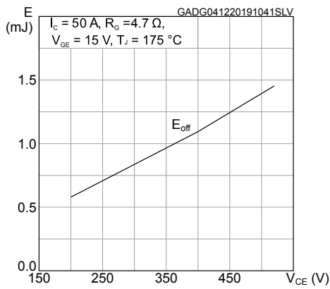
Figure 15. Switching energy vs collector emitter voltage
