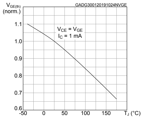
Figure 9. Normalized V_{GE(th)} vs junction temperature
