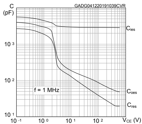
Figure 11. Capacitance variations
