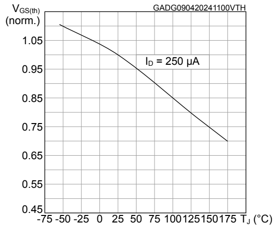
Figure 15. Normalized gate threshold voltage vs temperature
