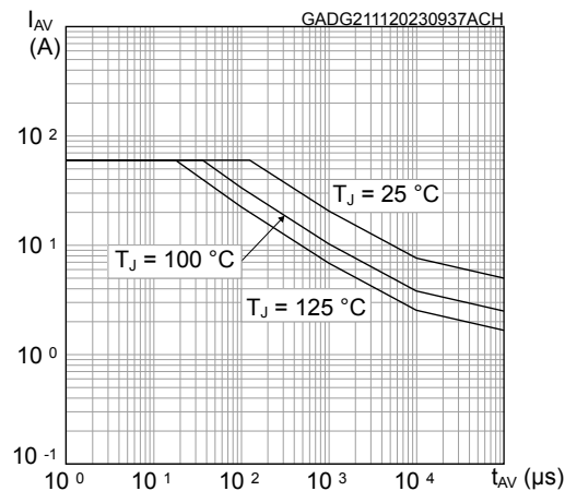
Figure 5. Avalanche characteristics
