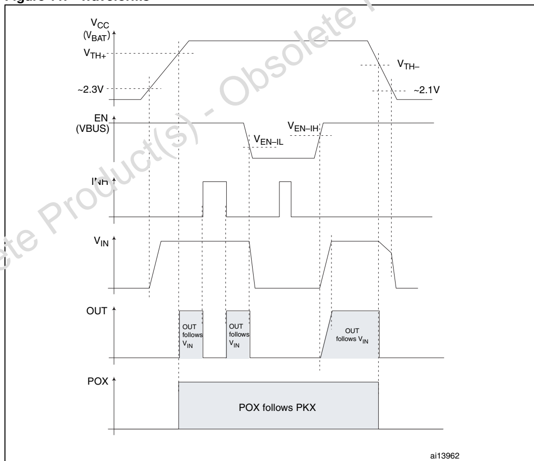
Figure 11. Waveforms
