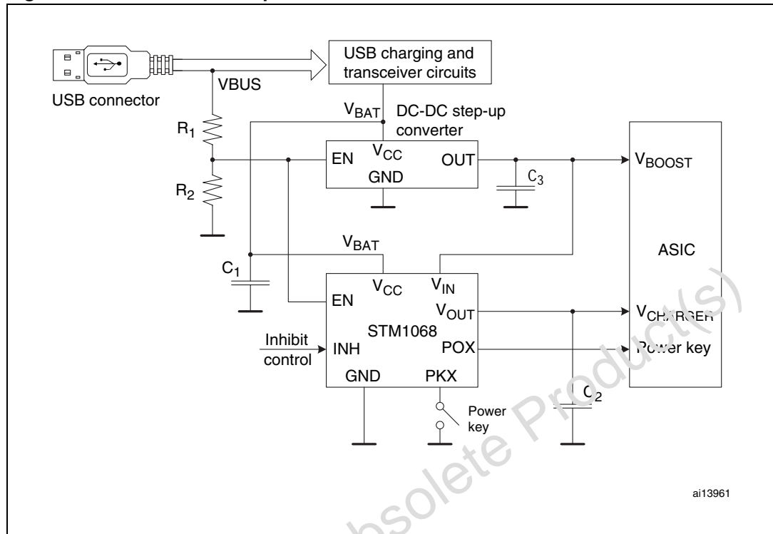
Figure 4. Hardware hookup
