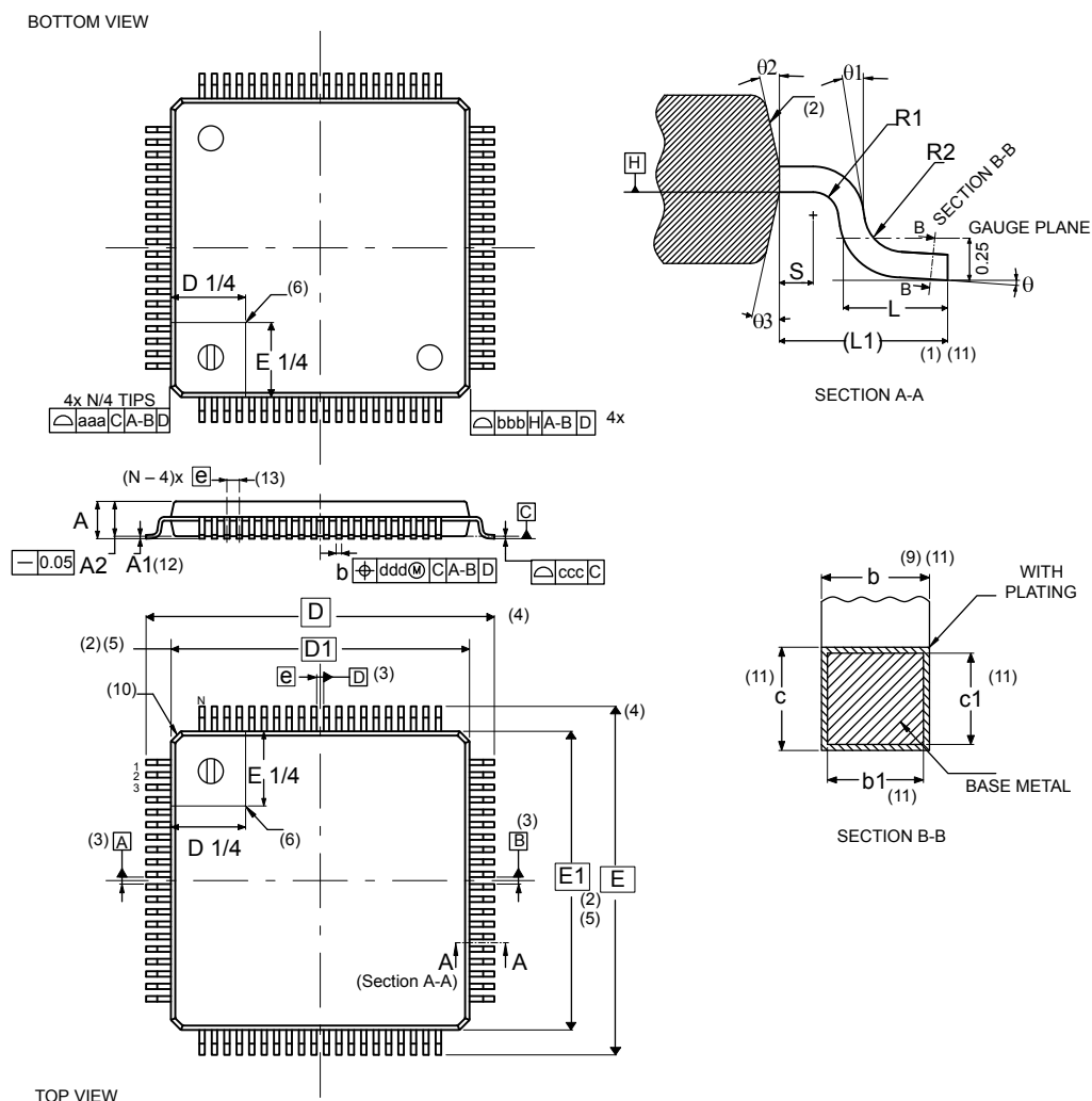
Figure 54. LQFP80 - Outline (15.)
