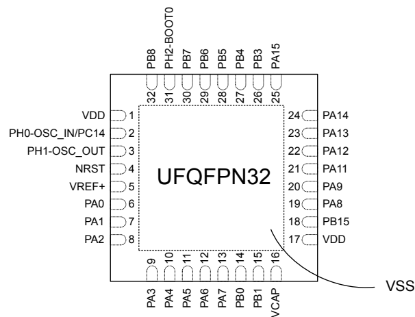
Figure 4. UFQFPN32 pinout
