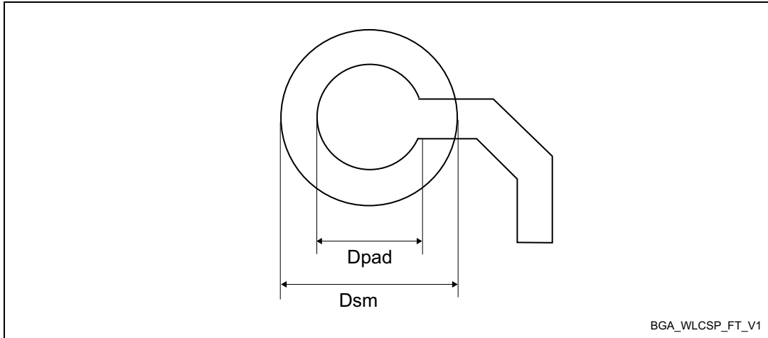
Figure 47. UFBGA64 – Footprint example
