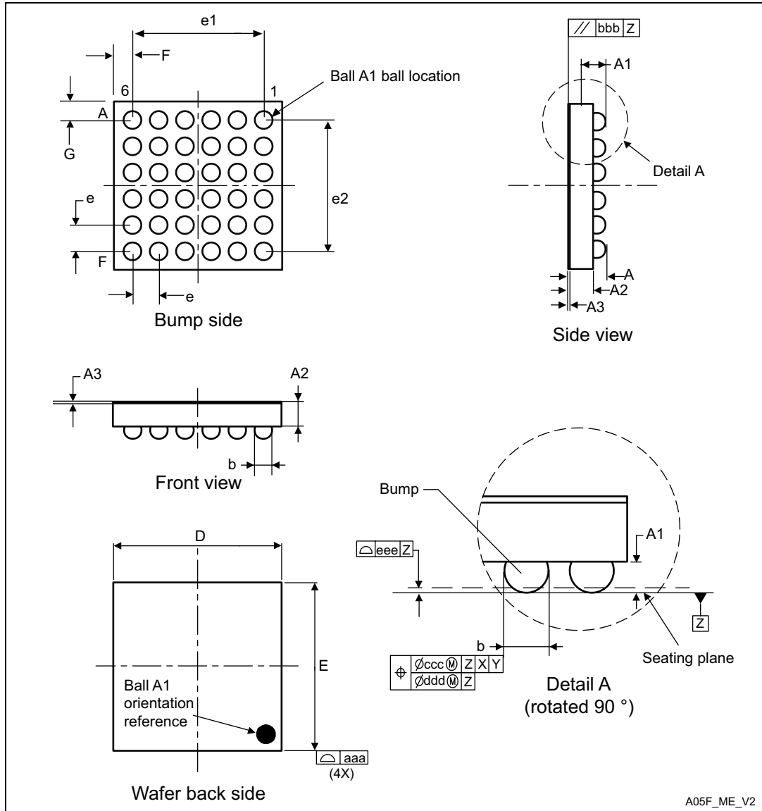
Figure 48. WLCSP36 - 36-ball, 2.553 x 2.579 mm, 0.4 mm pitch wafer level chip scale package outline
