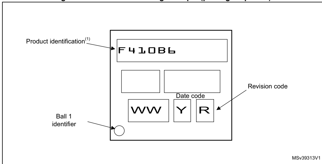
Figure 50. WLCSP36 marking example (package top view)
