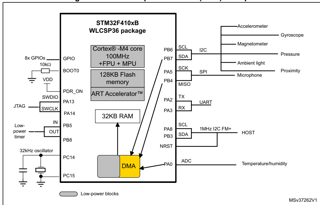
Figure 53. Batch Acquisition Mode (BAM) example
