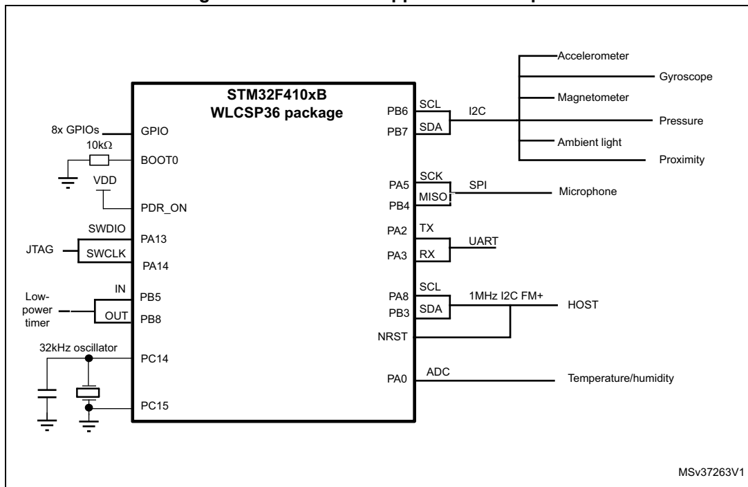
Figure 52. Sensor hub application example 2
