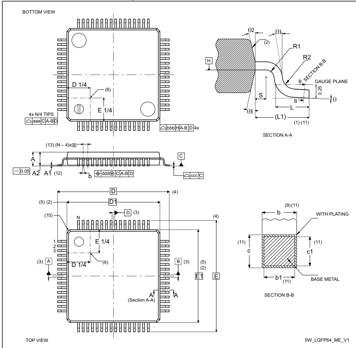
Figure 45. LQFP64 - Outline (15)
