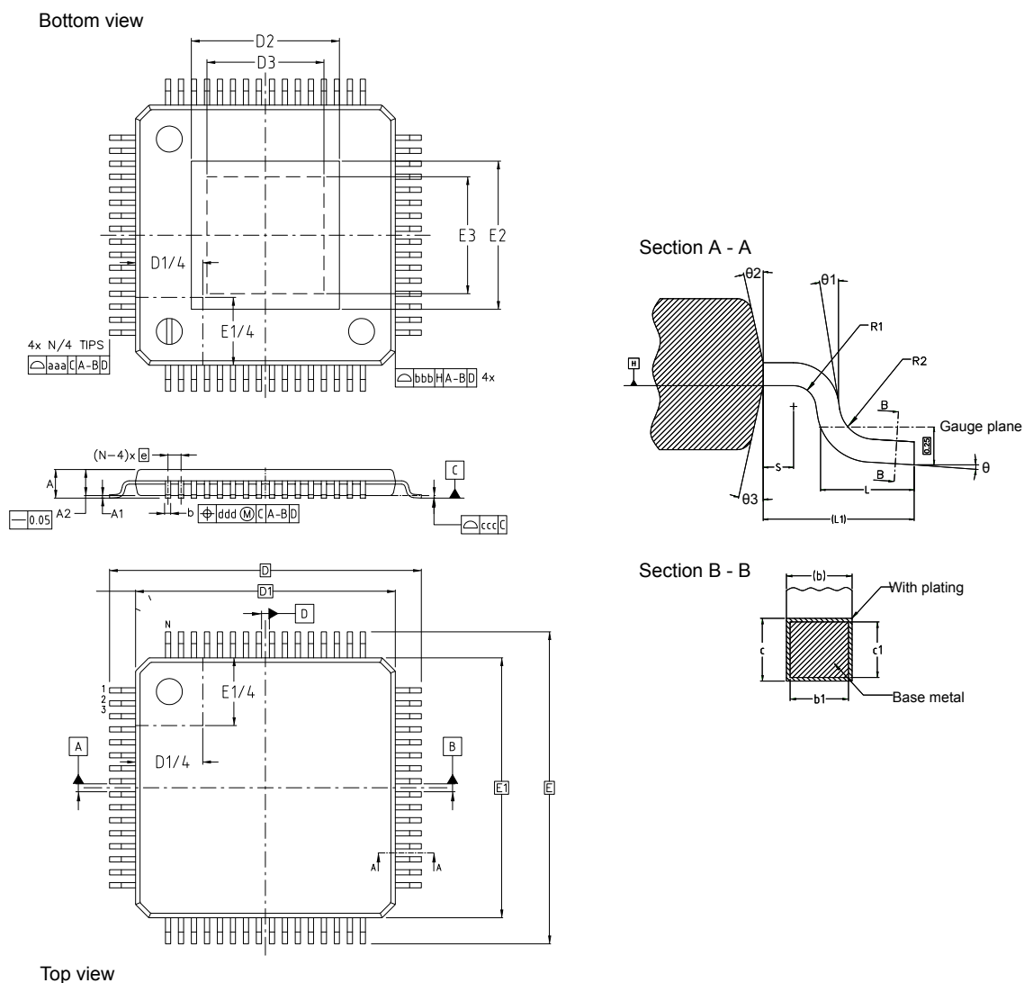
Figure 46. TQFP64-EP - Outline
