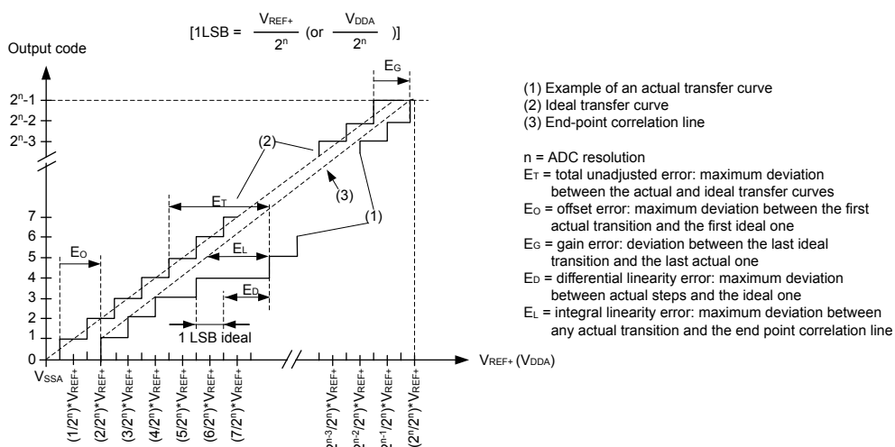
Figure 23. ADC accuracy characteristics
