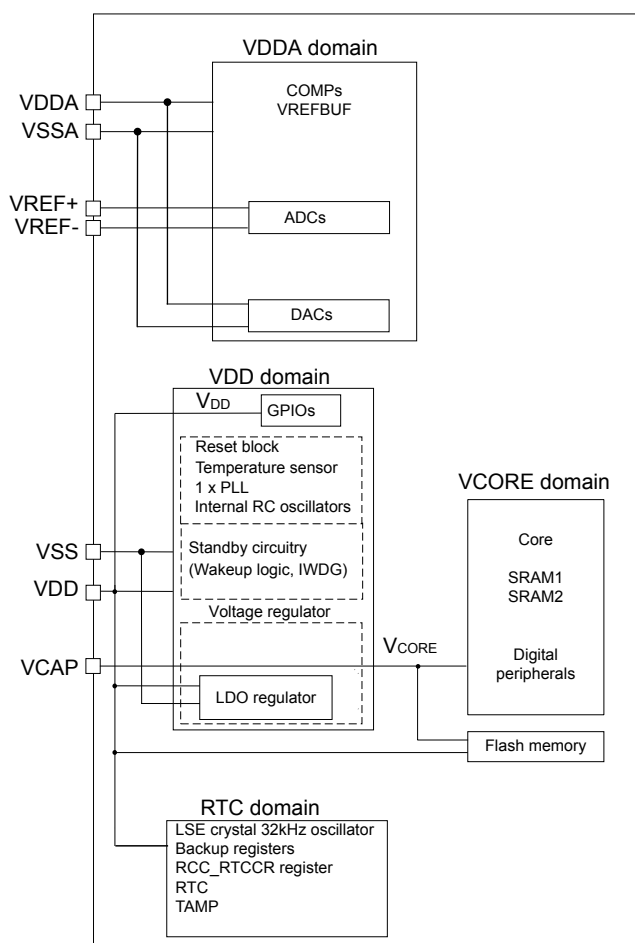
Figure 2. STM32G54xxx power supply overview (with LDO)
