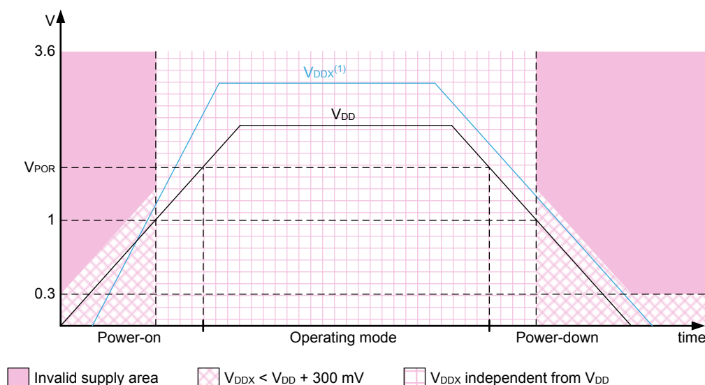
Figure 3. Power-up/down sequence
