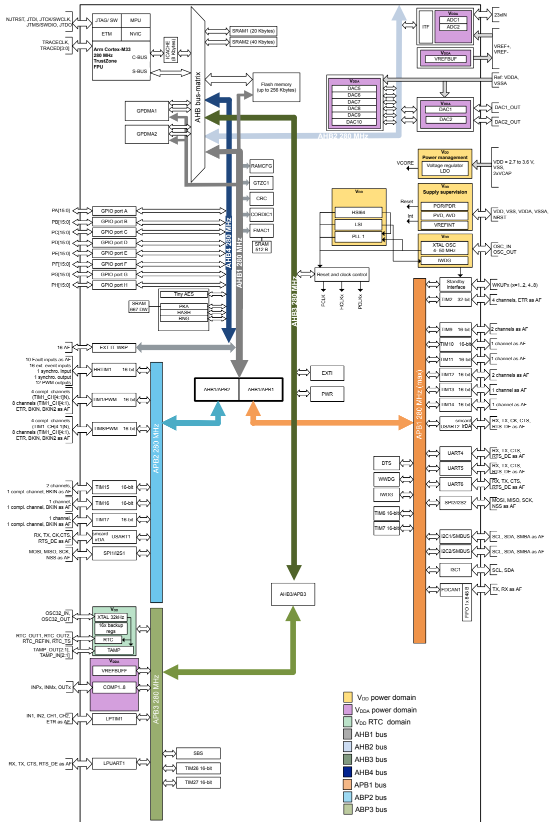
Figure 1. STM32G54xxx block diagram
