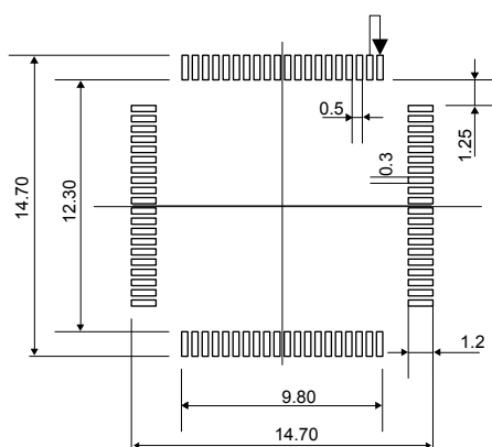
Figure 49. LQFP80 - Footprint example
