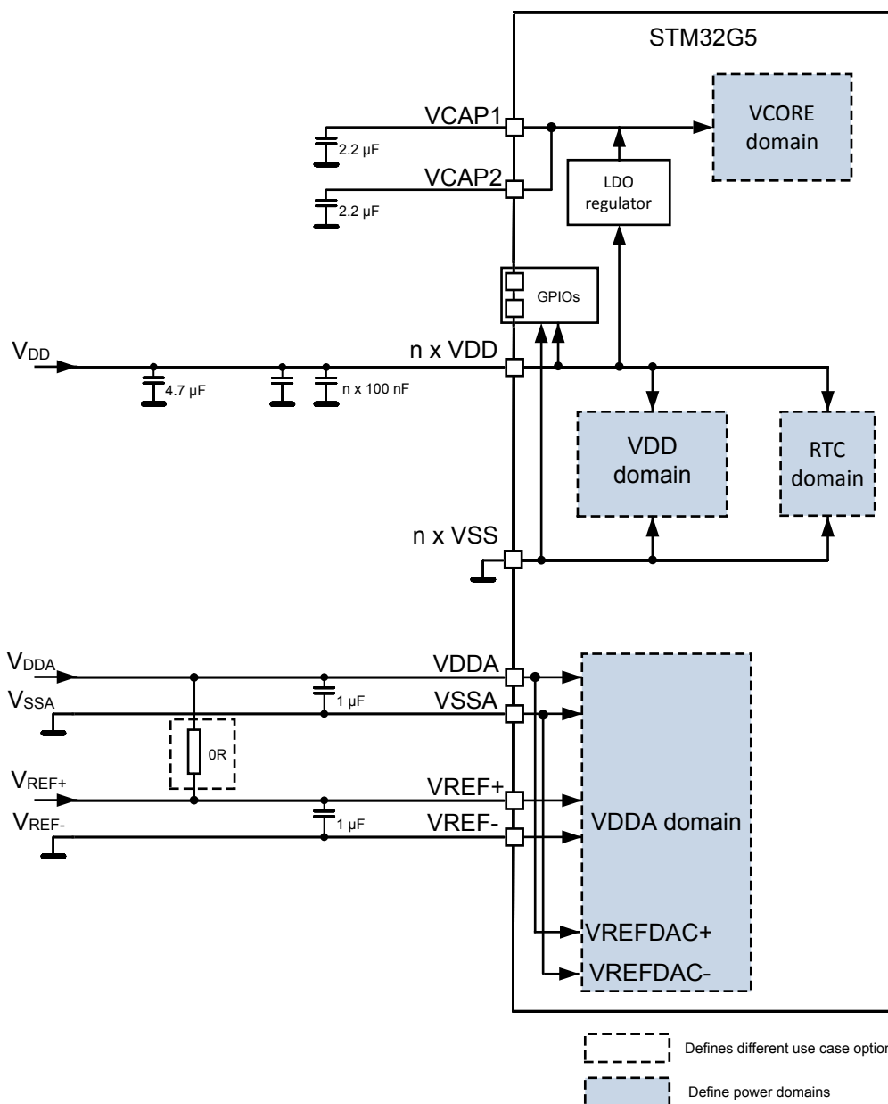
Figure 14. STM32G54xxx power supply scheme
