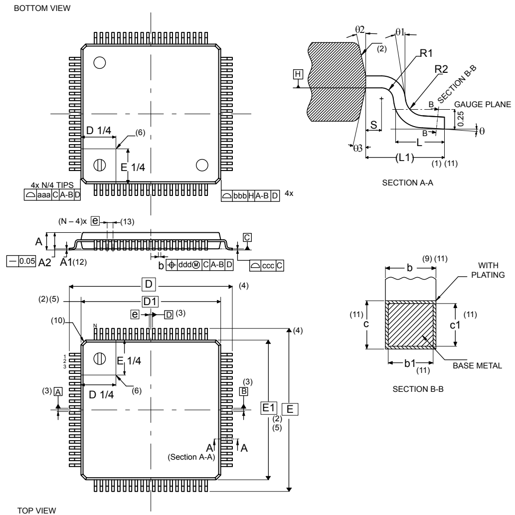
Figure 48. LQFP80 - Outline (15.)
