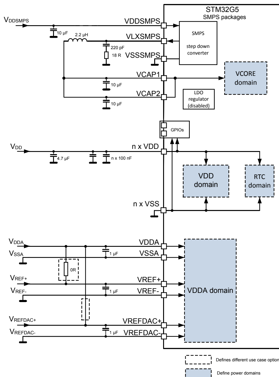
Figure 20. STM32G55xxx power supply scheme (with SMPS)
