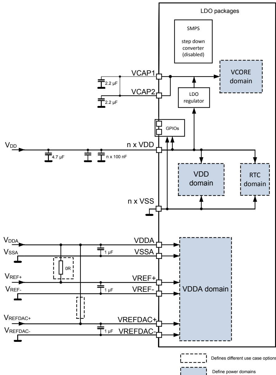
Figure 21. STM32G55xxx power supply scheme (with LDO)
