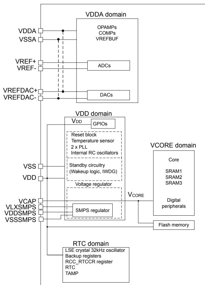
Figure 2. STM32G55xxx power supply overview (with SMPS)
