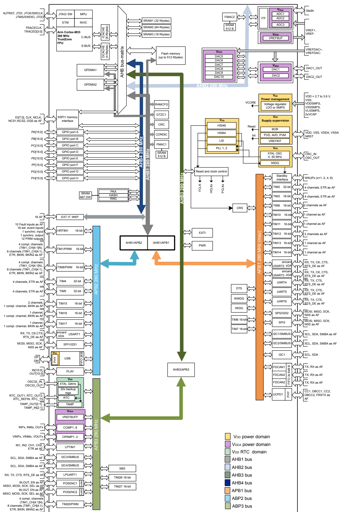
Figure 1. STM32G55xxx block diagram
