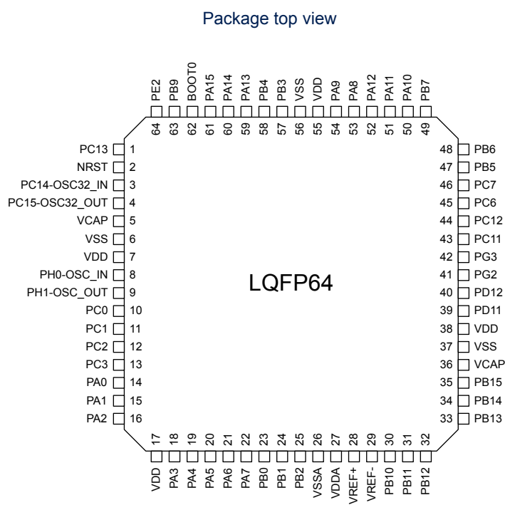
Figure 8. LQFP64 pinout
