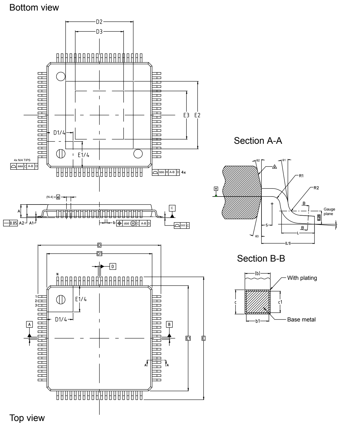
Figure 63. LQFP80-EP - Outline
