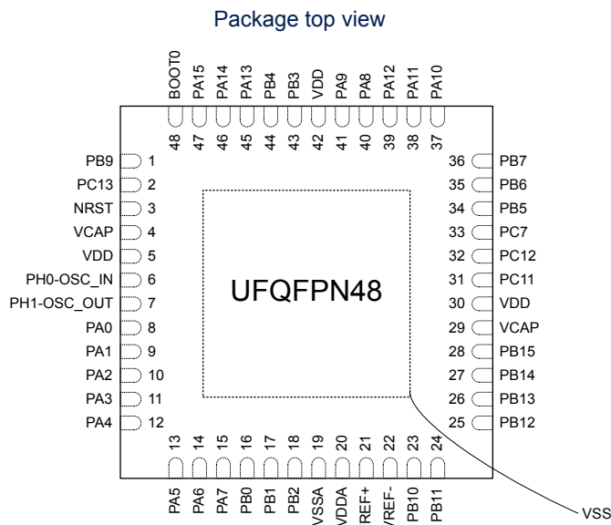
Figure 7. UFQFPN48 pinout
