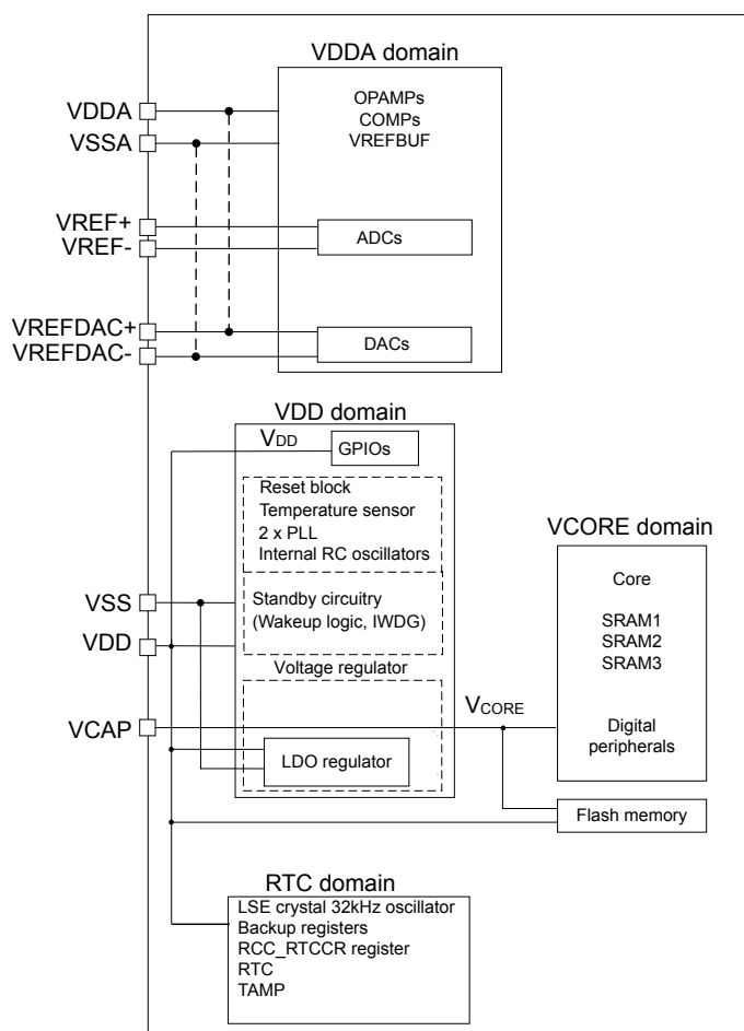
Figure 3. STM32G55xxx power supply overview (with LDO)
