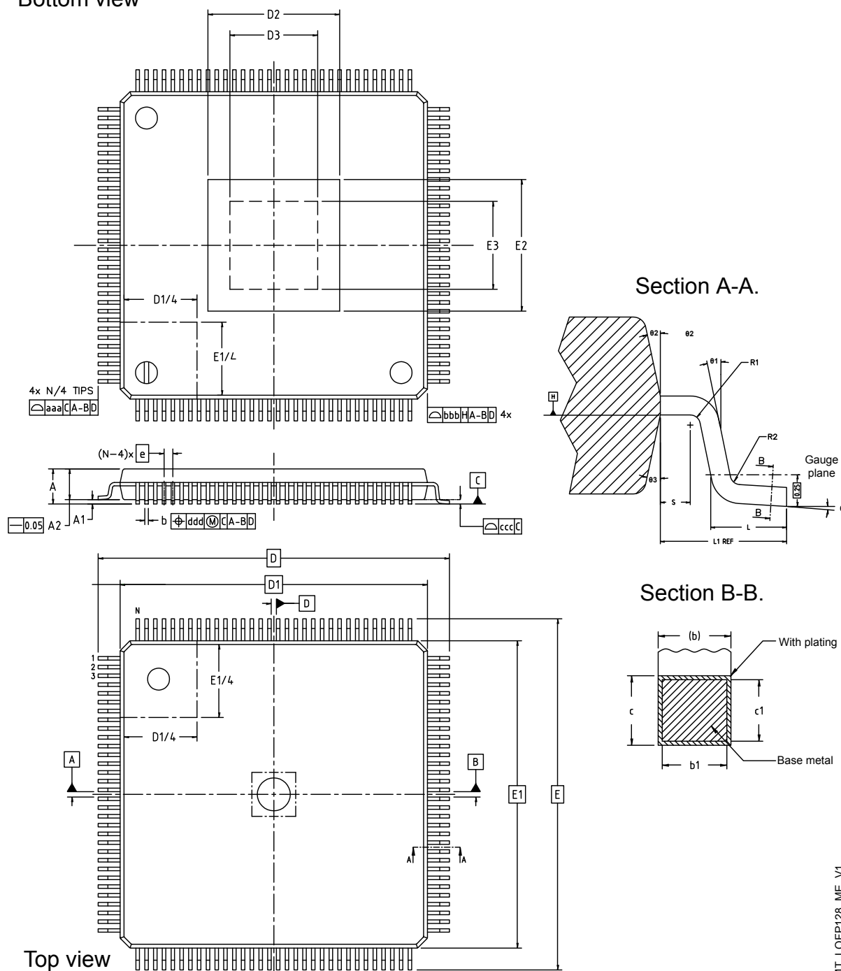
Figure 71. LQFP128-EP - Outline
