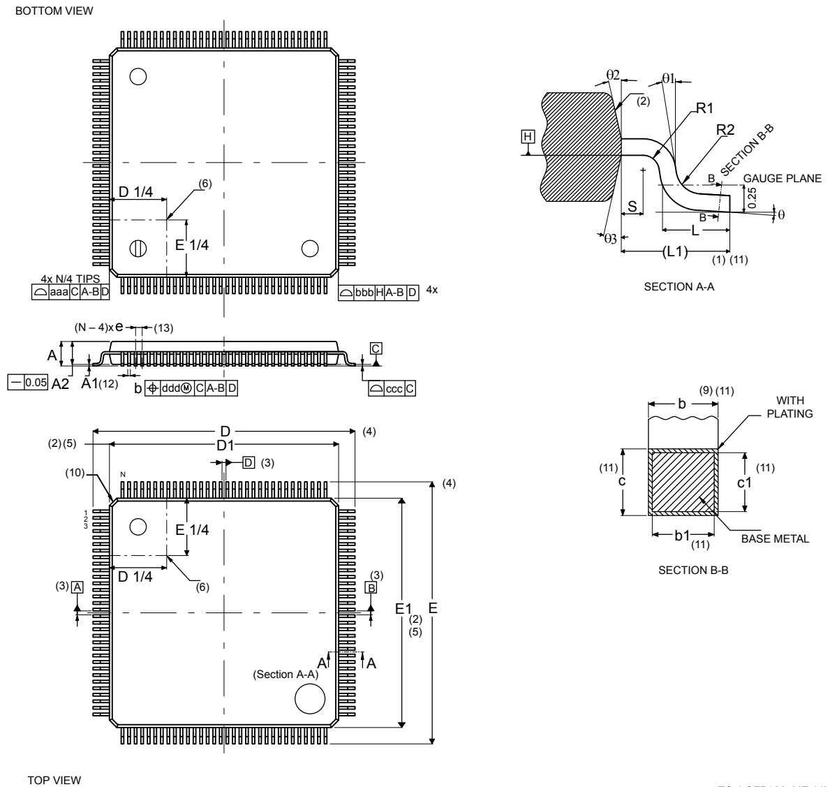
Figure 69. LQFP128 - Outline
