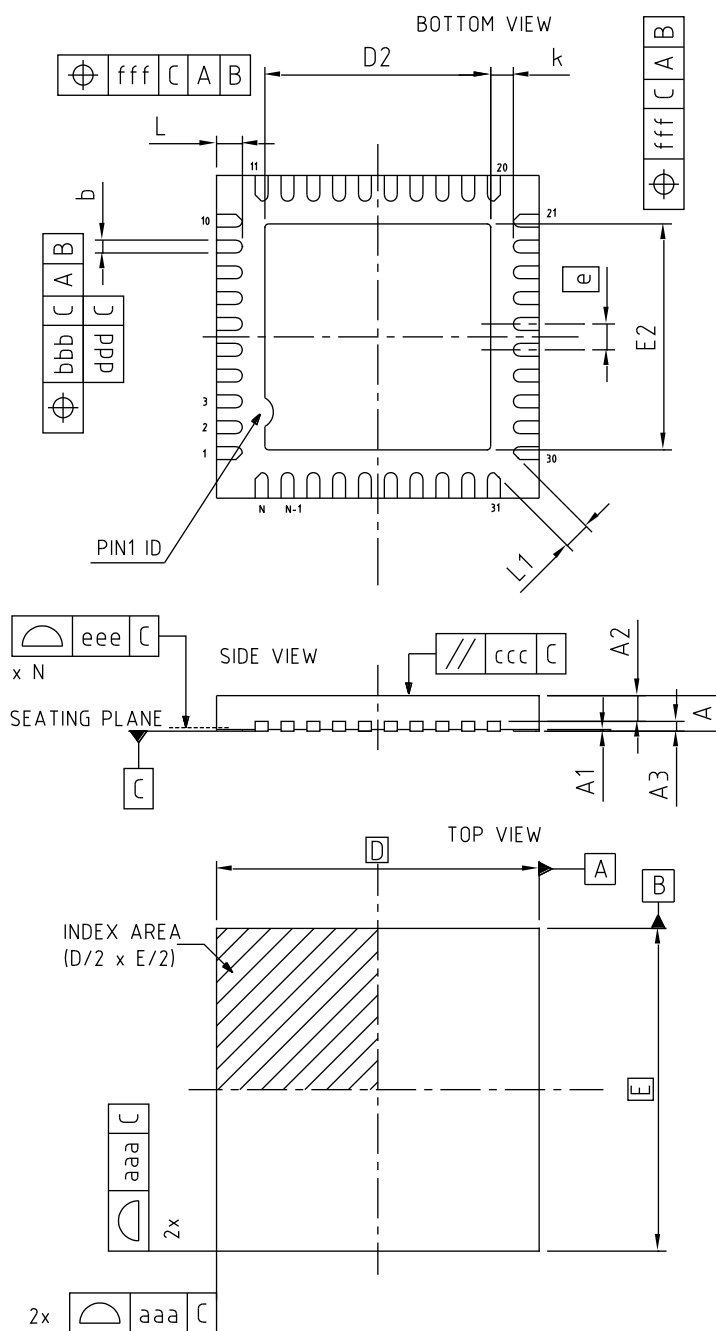
Figure 51. UFQFPN40 - Outline
