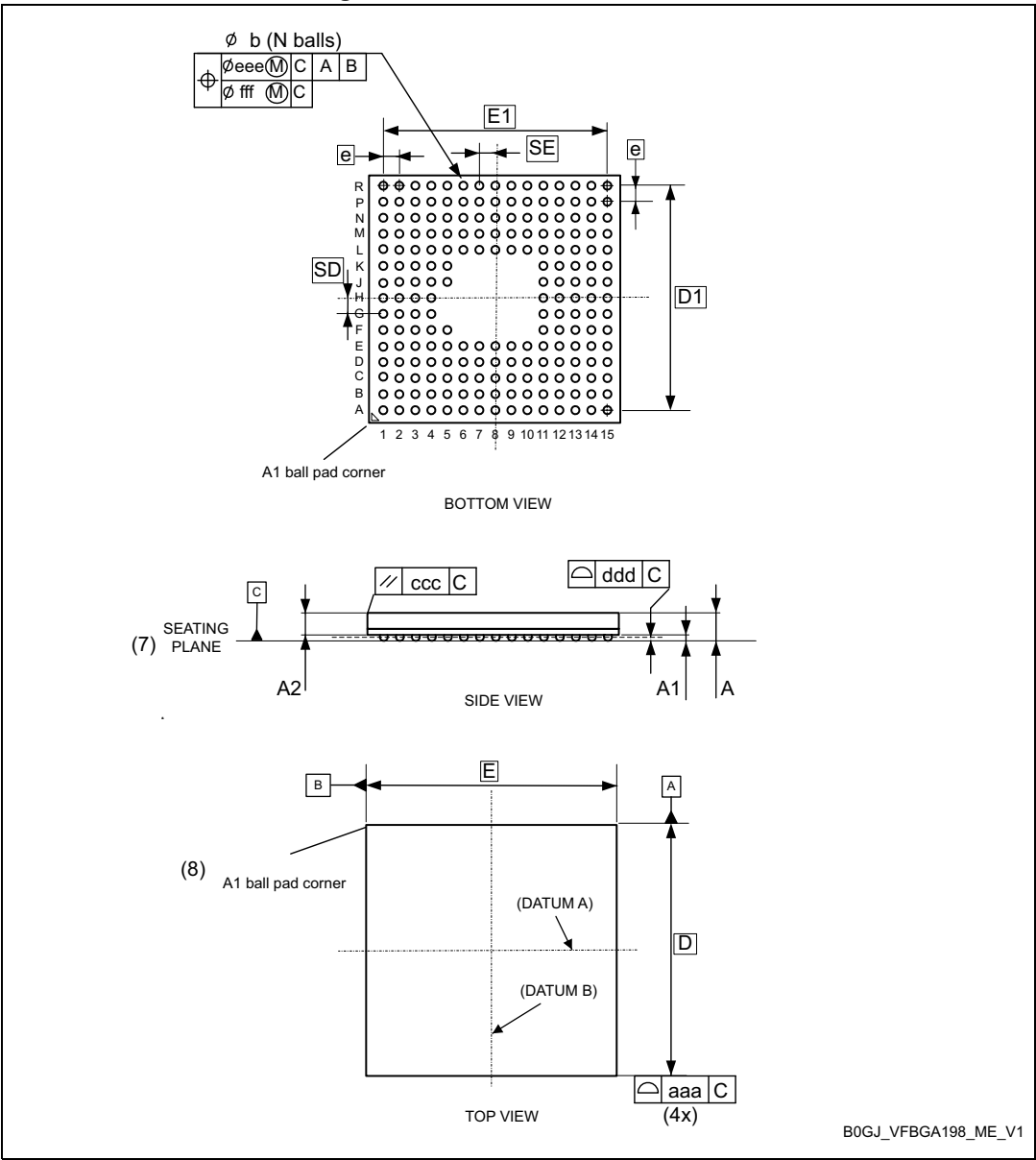
Figure 71. VFBGA198 - Outline (13)
