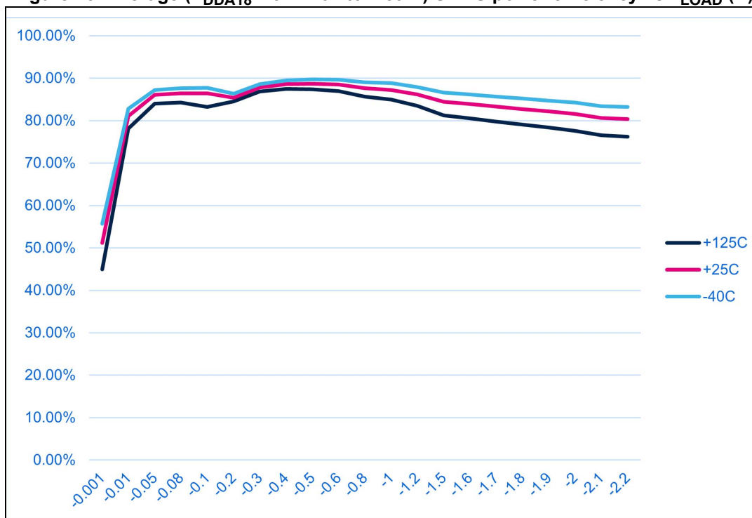
Figure 18. Average ( V_{DDA18} from 1.62 to 1.89 V) SMPS power efficiency vs. I_{LOAD} (A)
