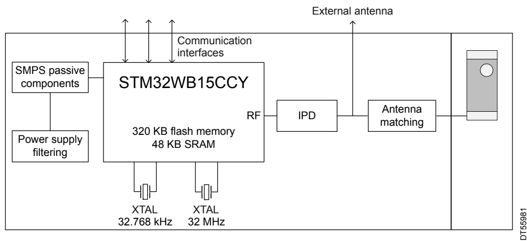
Figure 1. Block diagram
